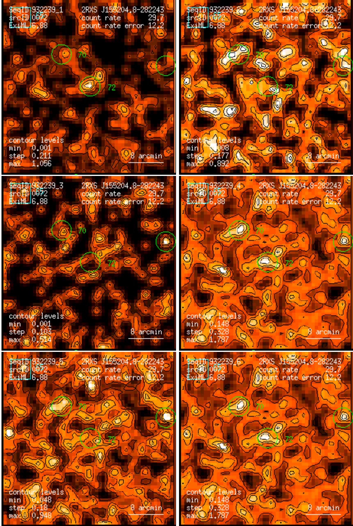
Figure 72: RASS 932239: detection 0072: band rate images, Gaussian filter: (1) PSPC channels 11 – 41, (2) 52 – 90, (3) 91 – 201, (4) 11 – 235, (5) 52 – 201, (6) 11 – 201. Broad band rates in counts/ks. Band rate contour levels in counts/ks/arcmin 2 .
