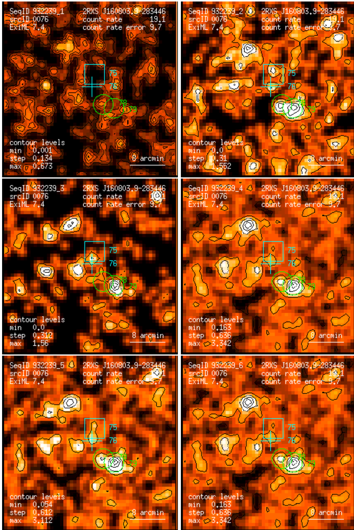
Figure 76: RASS 932239: detection 0076: band rate images, Gaussian filter: (1) PSPC channels 11 – 41, (2) 52 – 90, (3) 91 – 201, (4) 11 – 235, (5) 52 – 201, (6) 11 – 201. Broad band rates in counts/ks. Band rate contour levels in counts/ks/arcmin 2 .
