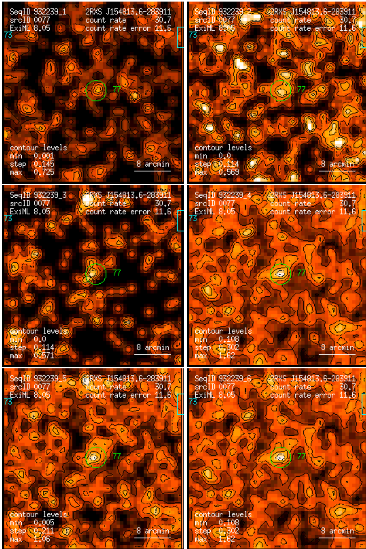
Figure 77: RASS 932239: detection 0077: band rate images, Gaussian filter: (1) PSPC channels 11 – 41, (2) 52 – 90, (3) 91 – 201, (4) 11 – 235, (5) 52 – 201, (6) 11 – 201. Broad band rates in counts/ks. Band rate contour levels in counts/ks/arcmin 2 .
