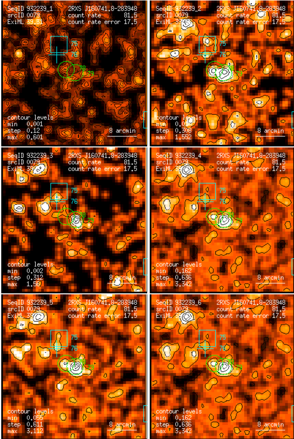
Figure 79: RASS 932239: detection 0079: band rate images, Gaussian filter: (1) PSPC channels 11 – 41, (2) 52 – 90, (3) 91 – 201, (4) 11 – 235, (5) 52 – 201, (6) 11 – 201. Broad band rates in counts/ks. Band rate contour levels in counts/ks/arcmin 2 .
