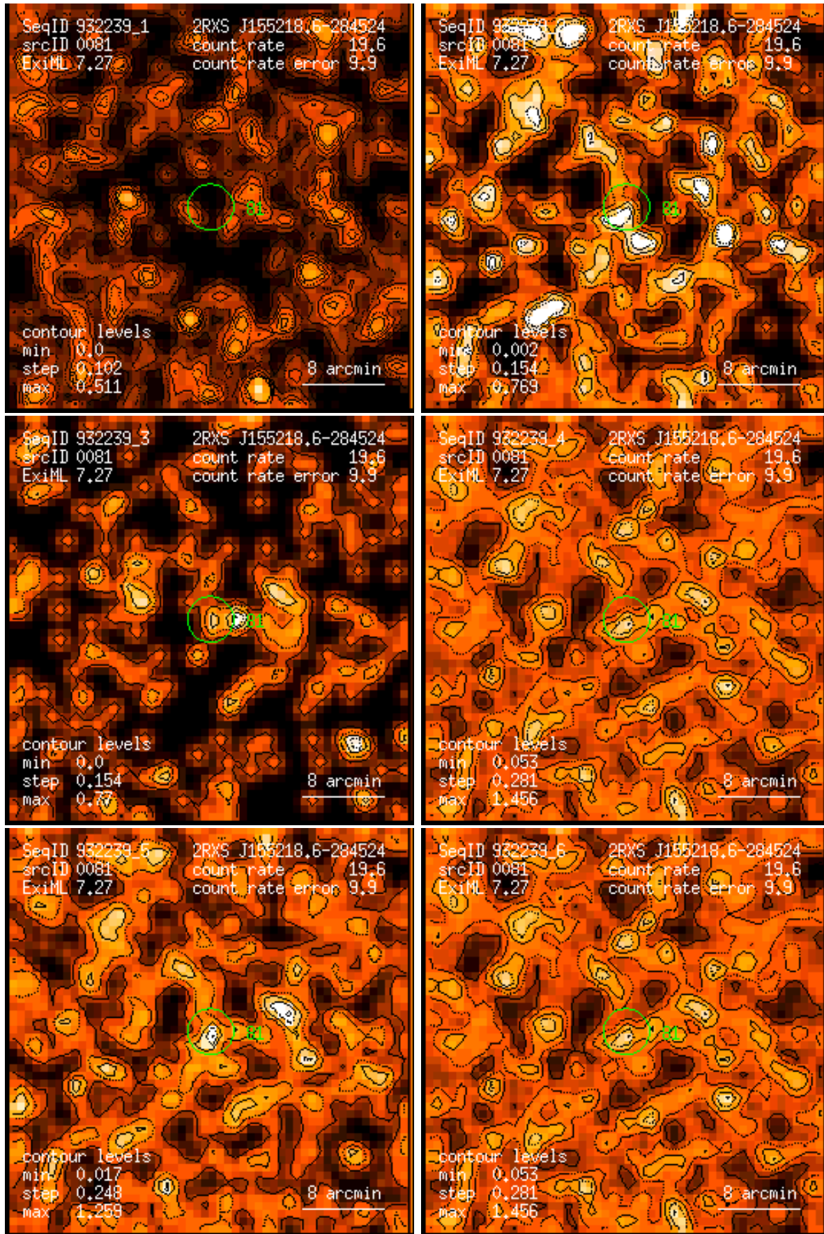
Figure 81: RASS 932239: detection 0081: band rate images, Gaussian filter: (1) PSPC channels 11 – 41, (2) 52 – 90, (3) 91 – 201, (4) 11 – 235, (5) 52 – 201, (6) 11 – 201. Broad band rates in counts/ks. Band rate contour levels in counts/ks/arcmin 2 .
