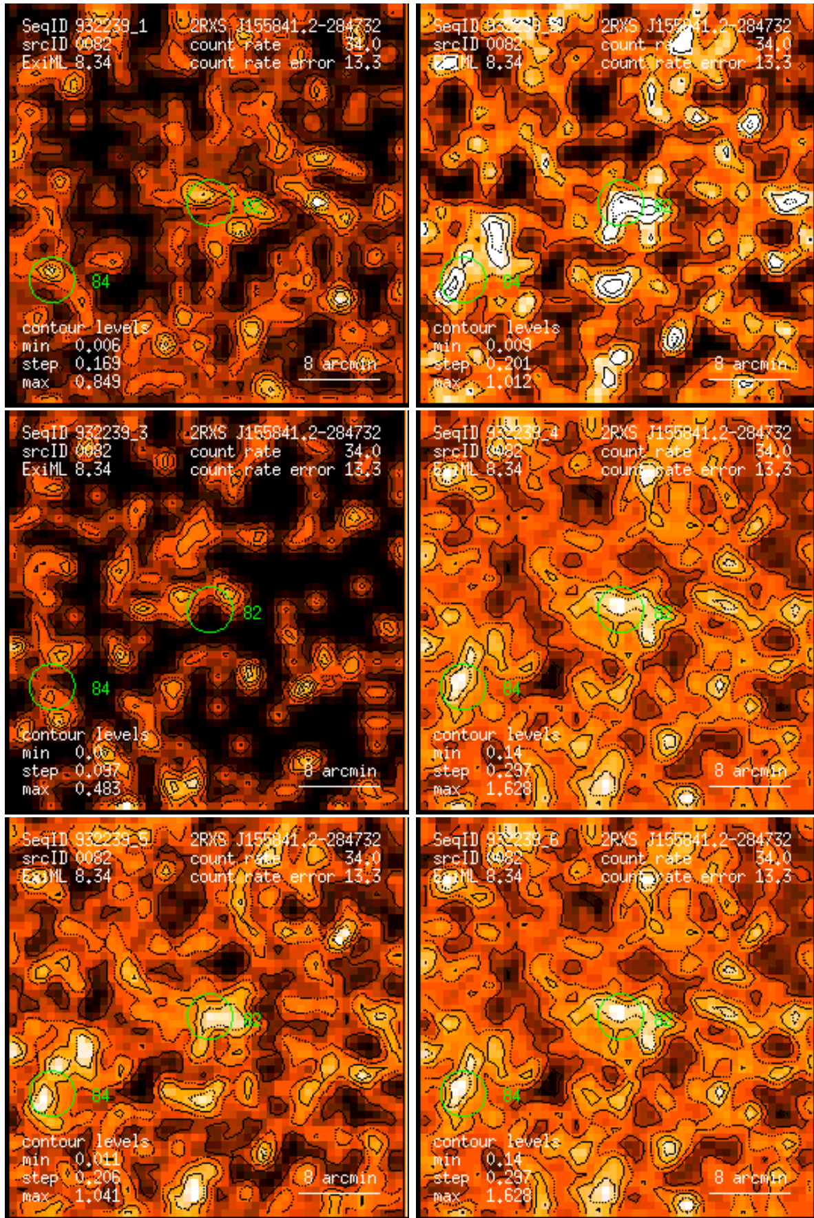
Figure 82: RASS 932239: detection 0082: band rate images, Gaussian filter: (1) PSPC channels 11 – 41, (2) 52 – 90, (3) 91 – 201, (4) 11 – 235, (5) 52 – 201, (6) 11 – 201. Broad band rates in counts/ks. Band rate contour levels in counts/ks/arcmin 2 .
