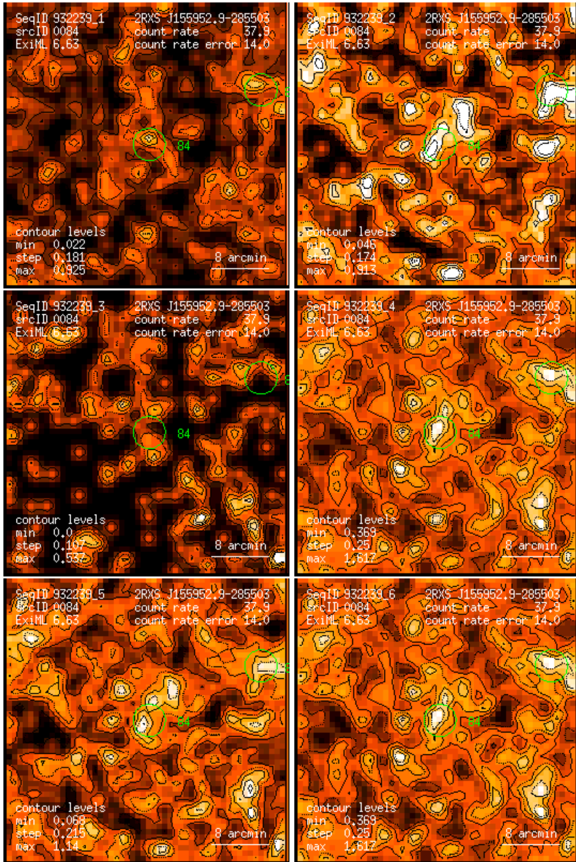
Figure 84: RASS 932239: detection 0084: band rate images, Gaussian filter: (1) PSPC channels 11 – 41, (2) 52 – 90, (3) 91 – 201, (4) 11 – 235, (5) 52 – 201, (6) 11 – 201. Broad band rates in counts/ks. Band rate contour levels in counts/ks/arcmin 2 .
