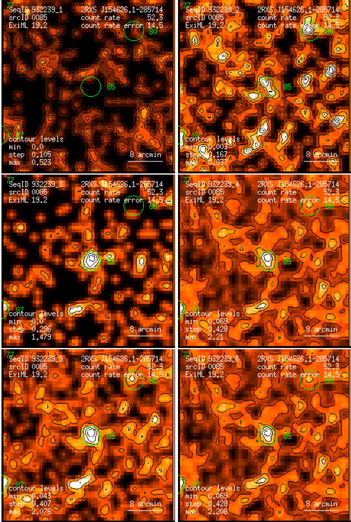
Figure 85: RASS 932239: detection 0085: band rate images, Gaussian filter: (1) PSPC channels 11 – 41, (2) 52 – 90, (3) 91 – 201, (4) 11 – 235, (5) 52 – 201, (6) 11 – 201. Broad band rates in counts/ks. Band rate contour levels in counts/ks/arcmin 2 .
