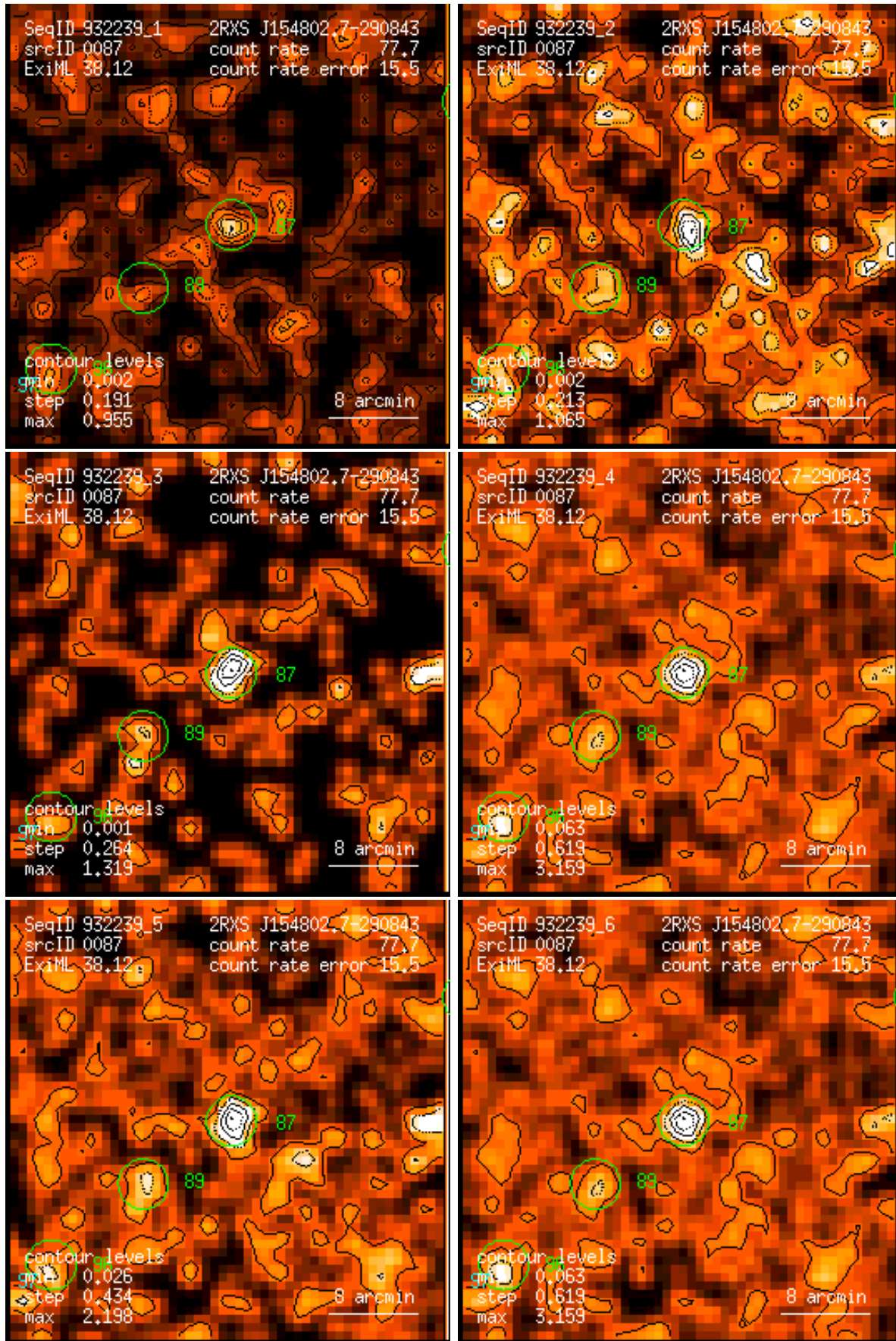
Figure 87: RASS 932239: detection 0087: band rate images, Gaussian filter: (1) PSPC channels 11 – 41, (2) 52 – 90, (3) 91 – 201, (4) 11 – 235, (5) 52 – 201, (6) 11 – 201. Broad band rates in counts/ks. Band rate contour levels in counts/ks/arcmin 2 .
