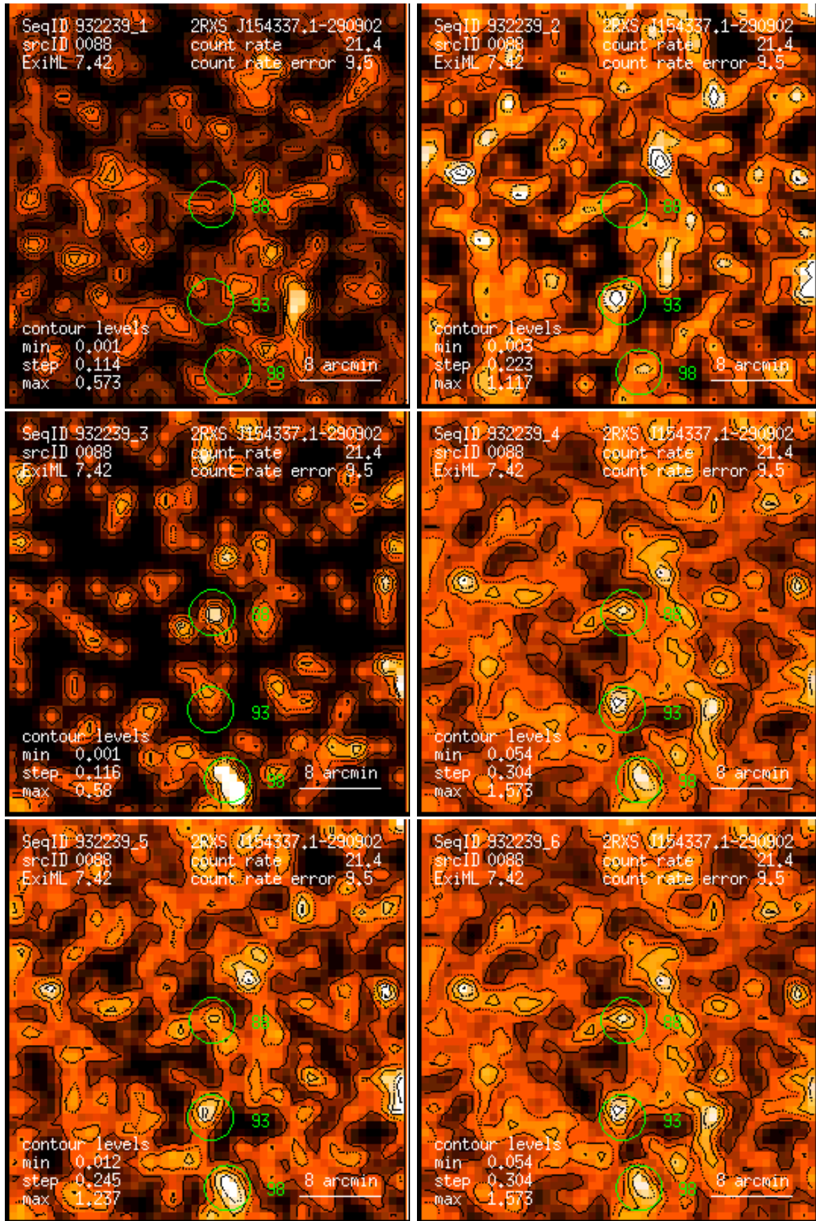
Figure 88: RASS 932239: detection 0088: band rate images, Gaussian filter: (1) PSPC channels 11 – 41, (2) 52 – 90, (3) 91 – 201, (4) 11 – 235, (5) 52 – 201, (6) 11 – 201. Broad band rates in counts/ks. Band rate contour levels in counts/ks/arcmin 2 .
