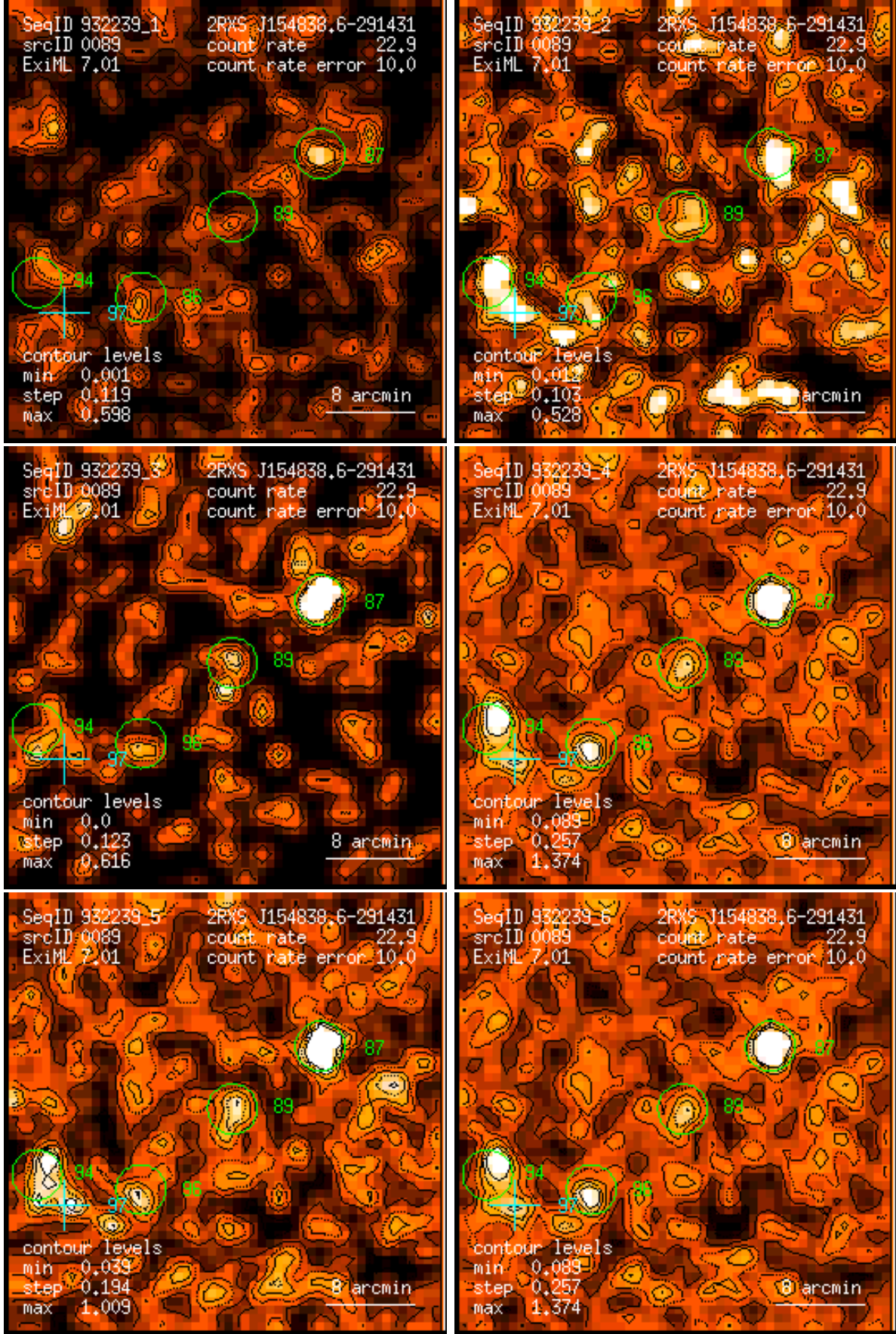
Figure 89: RASS 932239: detection 0089: band rate images, Gaussian filter: (1) PSPC channels 11 – 41, (2) 52 – 90, (3) 91 – 201, (4) 11 – 235, (5) 52 – 201, (6) 11 – 201. Broad band rates in counts/ks. Band rate contour levels in counts/ks/arcmin 2 .
