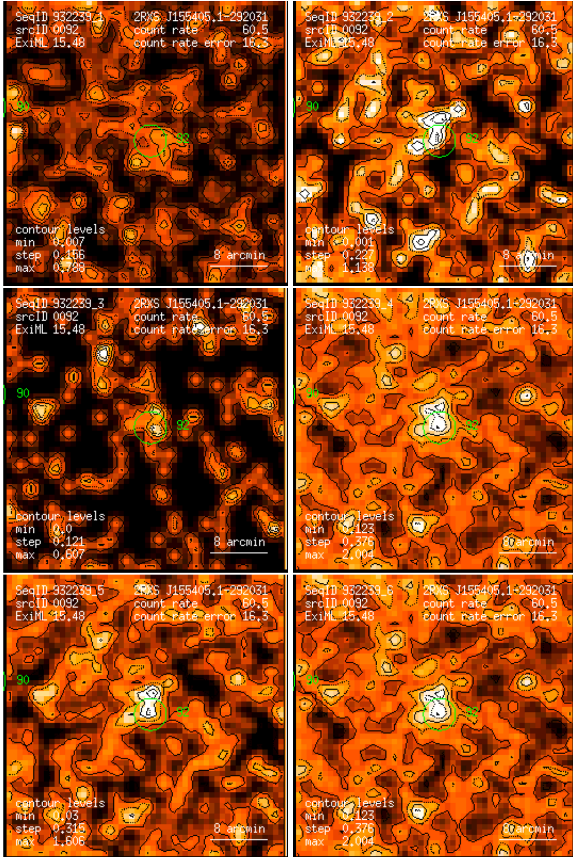
Figure 92: RASS 932239: detection 0092: band rate images, Gaussian filter: (1) PSPC channels 11 – 41, (2) 52 – 90, (3) 91 – 201, (4) 11 – 235, (5) 52 – 201, (6) 11 – 201. Broad band rates in counts/ks. Band rate contour levels in counts/ks/arcmin 2 .
