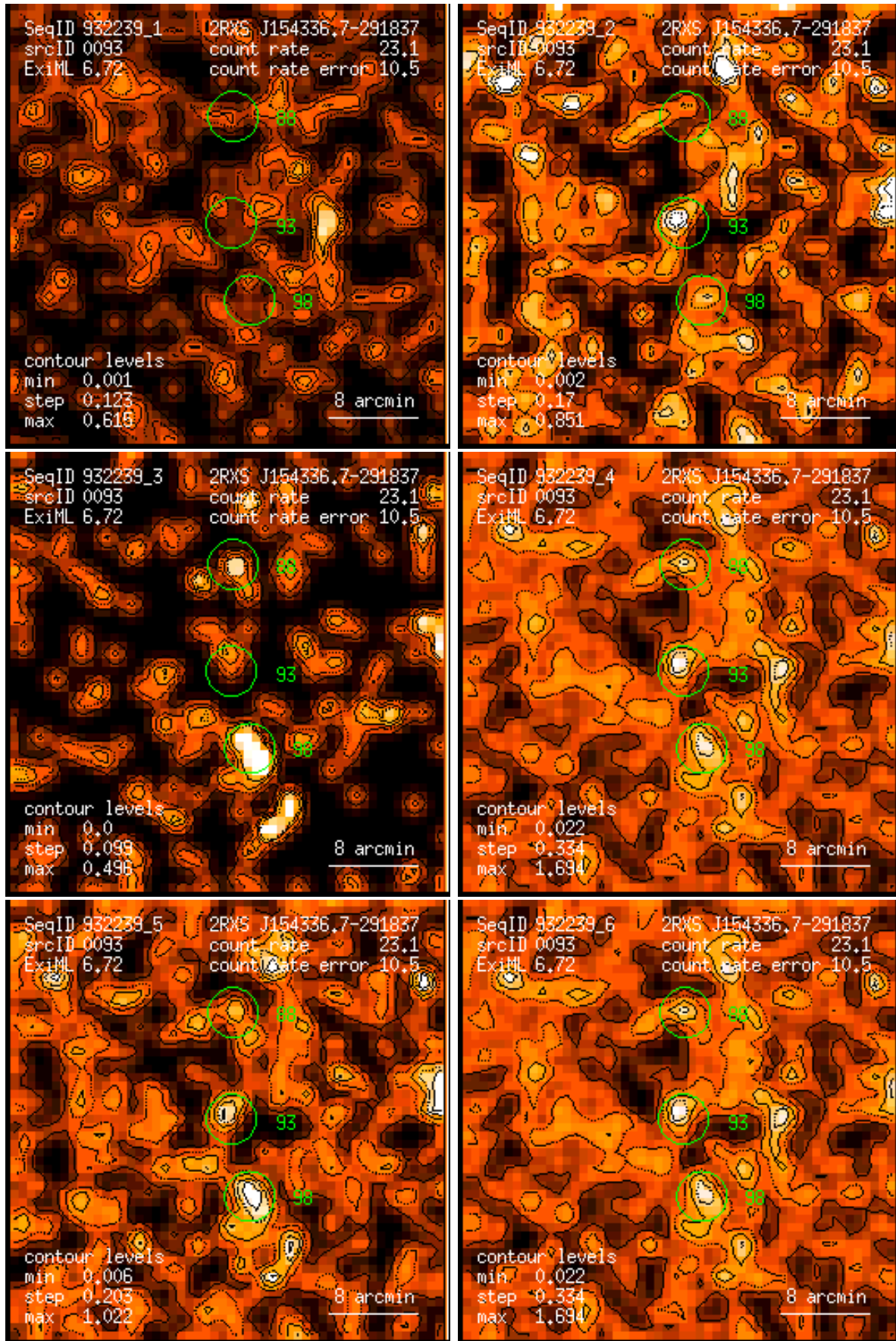
Figure 93: RASS 932239: detection 0093: band rate images, Gaussian filter: (1) PSPC channels 11 – 41, (2) 52 – 90, (3) 91 – 201, (4) 11 – 235, (5) 52 – 201, (6) 11 – 201. Broad band rates in counts/ks. Band rate contour levels in counts/ks/arcmin 2 .
