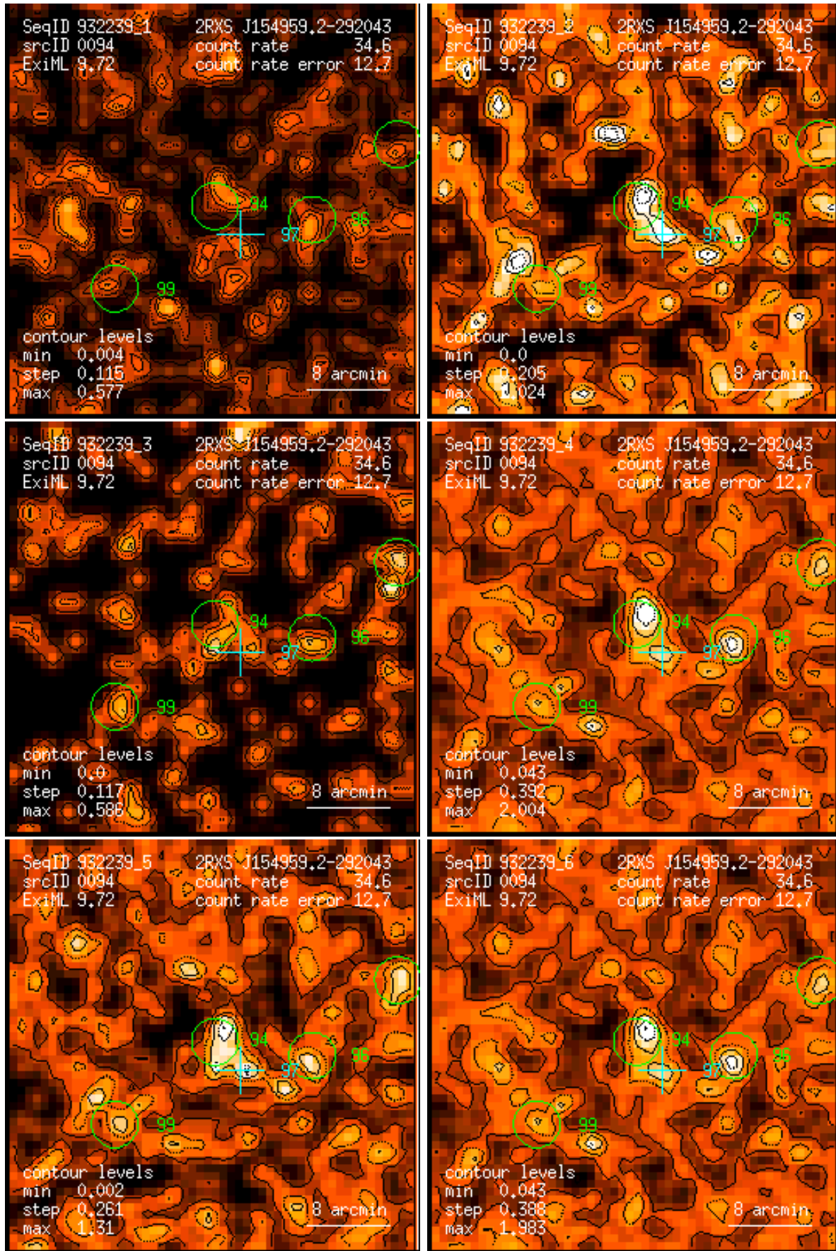
Figure 94: RASS 932239: detection 0094: band rate images, Gaussian filter: (1) PSPC channels 11 – 41, (2) 52 – 90, (3) 91 – 201, (4) 11 – 235, (5) 52 – 201, (6) 11 – 201. Broad band rates in counts/ks. Band rate contour levels in counts/ks/arcmin 2 .
