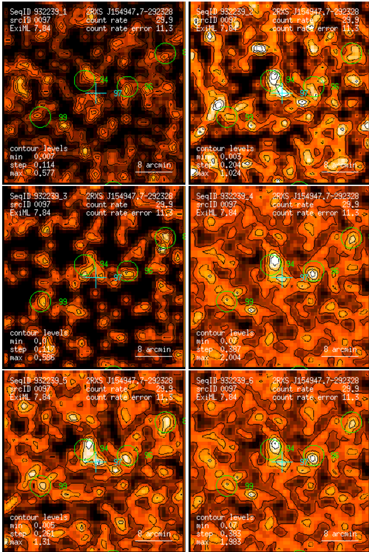
Figure 97: RASS 932239: detection 0097: band rate images, Gaussian filter: (1) PSPC channels 11 – 41, (2) 52 – 90, (3) 91 – 201, (4) 11 – 235, (5) 52 – 201, (6) 11 – 201. Broad band rates in counts/ks. Band rate contour levels in counts/ks/arcmin 2 .
