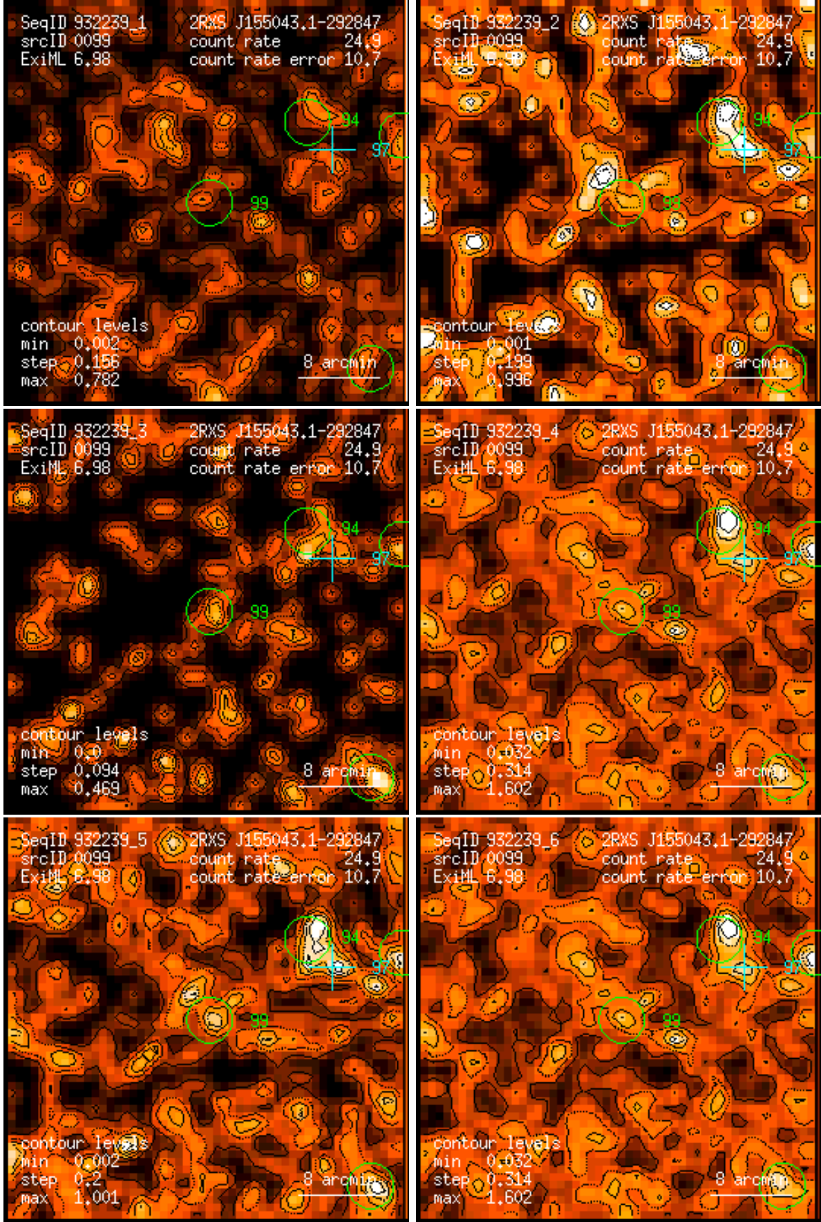
Figure 99: RASS 932239: detection 0099: band rate images, Gaussian filter: (1) PSPC channels 11 – 41, (2) 52 – 90, (3) 91 – 201, (4) 11 – 235, (5) 52 – 201, (6) 11 – 201. Broad band rates in counts/ks. Band rate contour levels in counts/ks/arcmin 2 .
