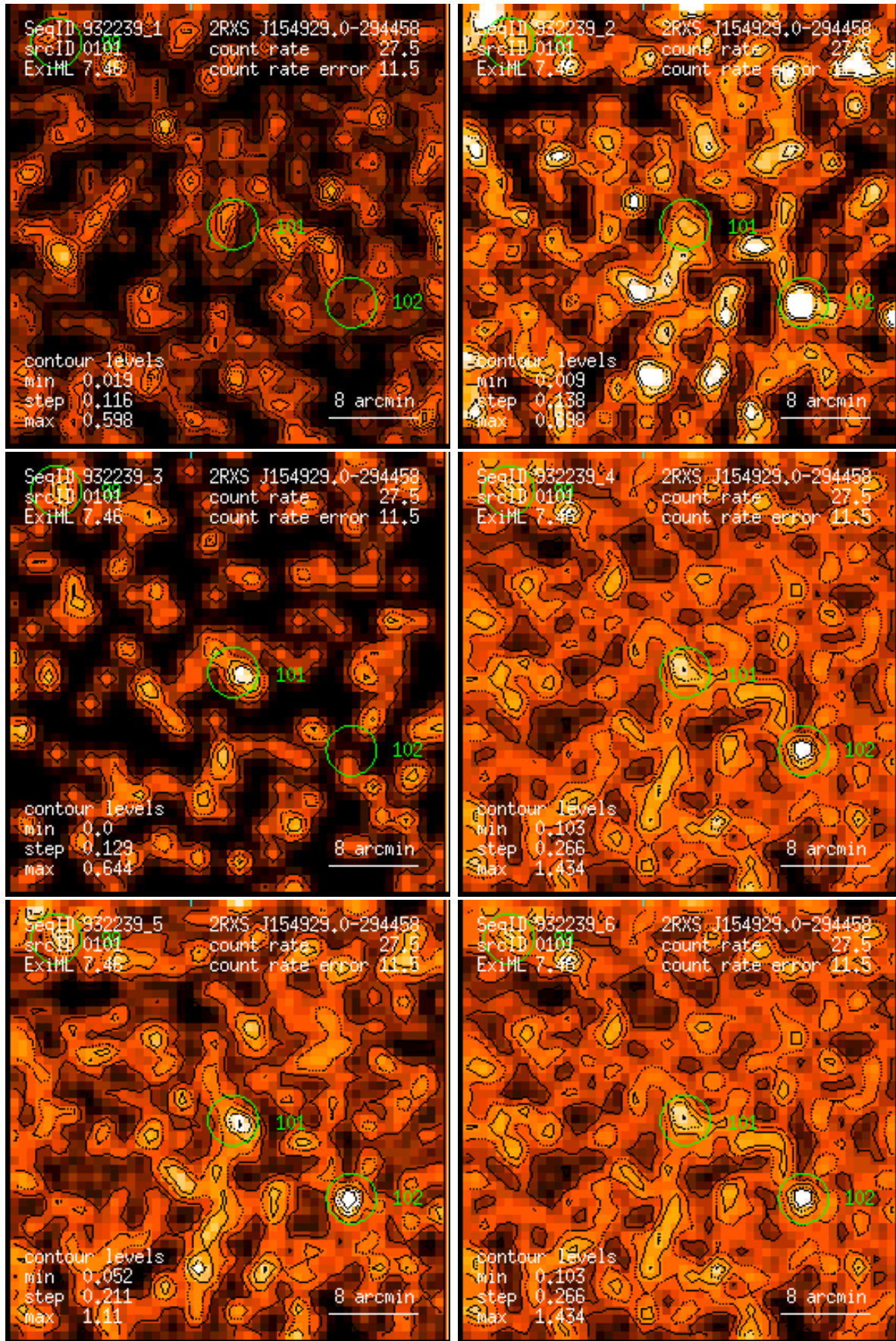
Figure 101: RASS 932239: detection 0101: band rate images, Gaussian filter: (1) PSPC channels 11 – 41, (2) 52 – 90, (3) 91 – 201, (4) 11 – 235, (5) 52 – 201, (6) 11 – 201. Broad band rates in counts/ks. Band rate contour levels in counts/ks/arcmin 2 .
