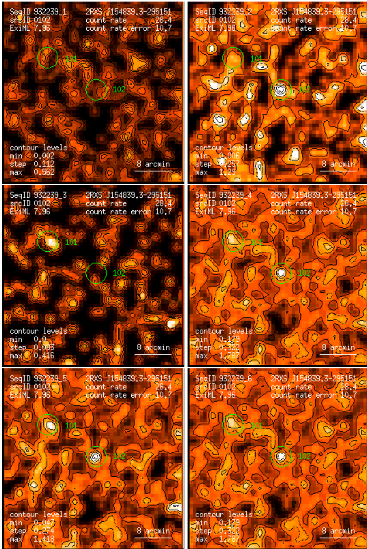
Figure 102: RASS 932239: detection 0102: band rate images, Gaussian filter: (1) PSPC channels 11 – 41, (2) 52 – 90, (3) 91 – 201, (4) 11 – 235, (5) 52 – 201, (6) 11 – 201. Broad band rates in counts/ks. Band rate contour levels in counts/ks/arcmin 2 .
