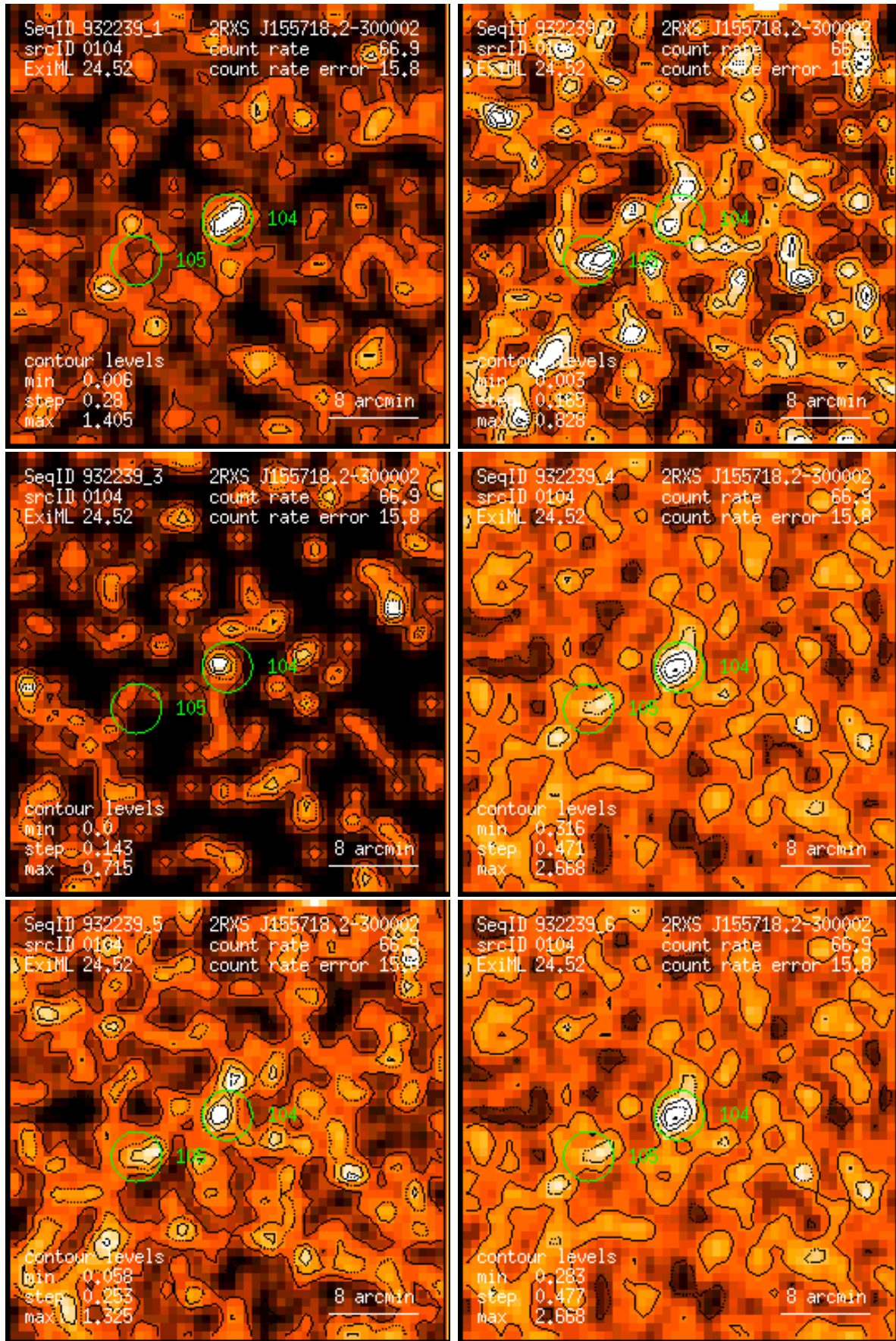
Figure 104: RASS 932239: detection 0104: band rate images, Gaussian filter: (1) PSPC channels 11 – 41, (2) 52 – 90, (3) 91 – 201, (4) 11 – 235, (5) 52 – 201, (6) 11 – 201. Broad band rates in counts/ks. Band rate contour levels in counts/ks/arcmin 2 .
