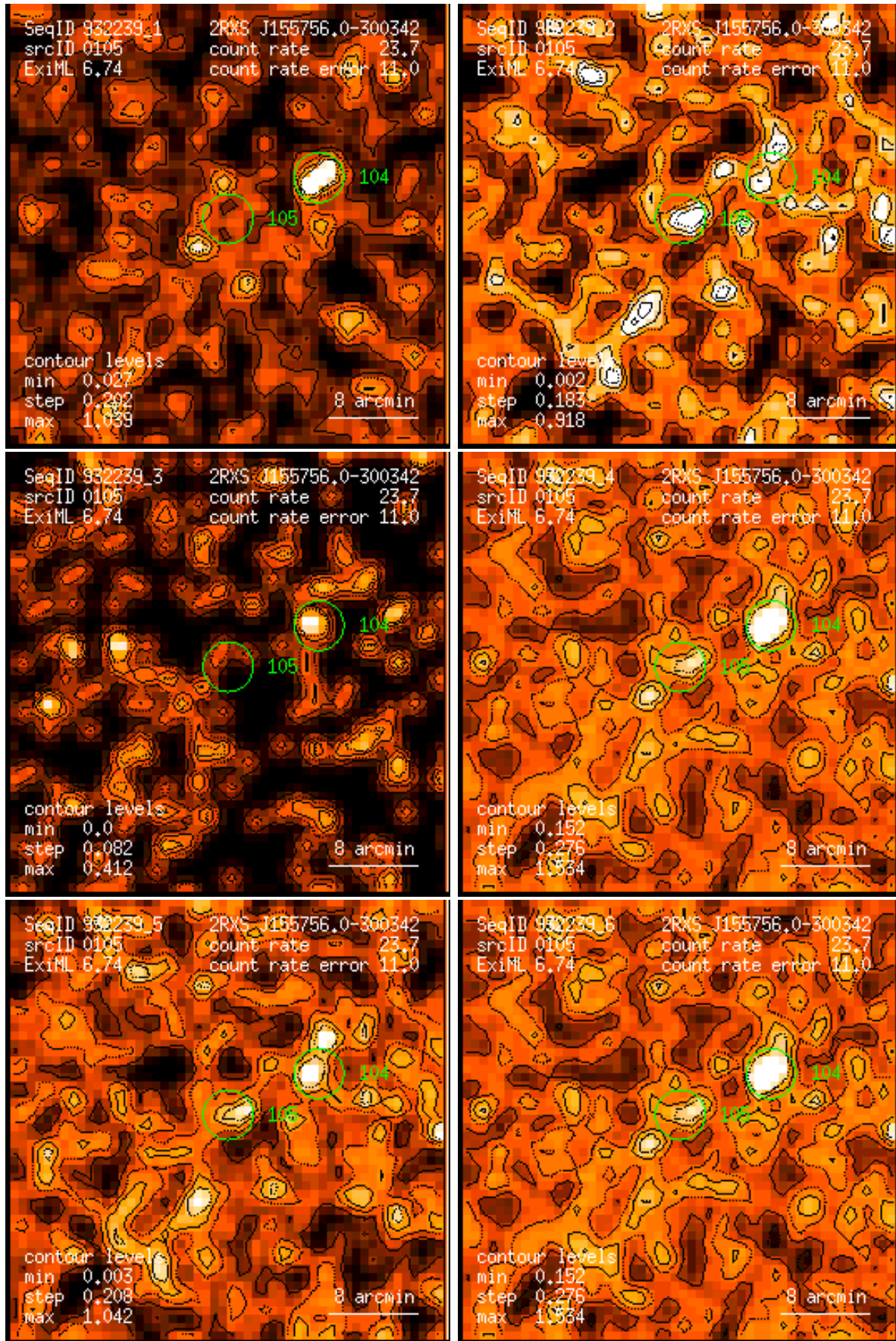
Figure 105: RASS 932239: detection 0105: band rate images, Gaussian filter: (1) PSPC channels 11 – 41, (2) 52 – 90, (3) 91 – 201, (4) 11 – 235, (5) 52 – 201, (6) 11 – 201. Broad band rates in counts/ks. Band rate contour levels in counts/ks/arcmin 2 .
