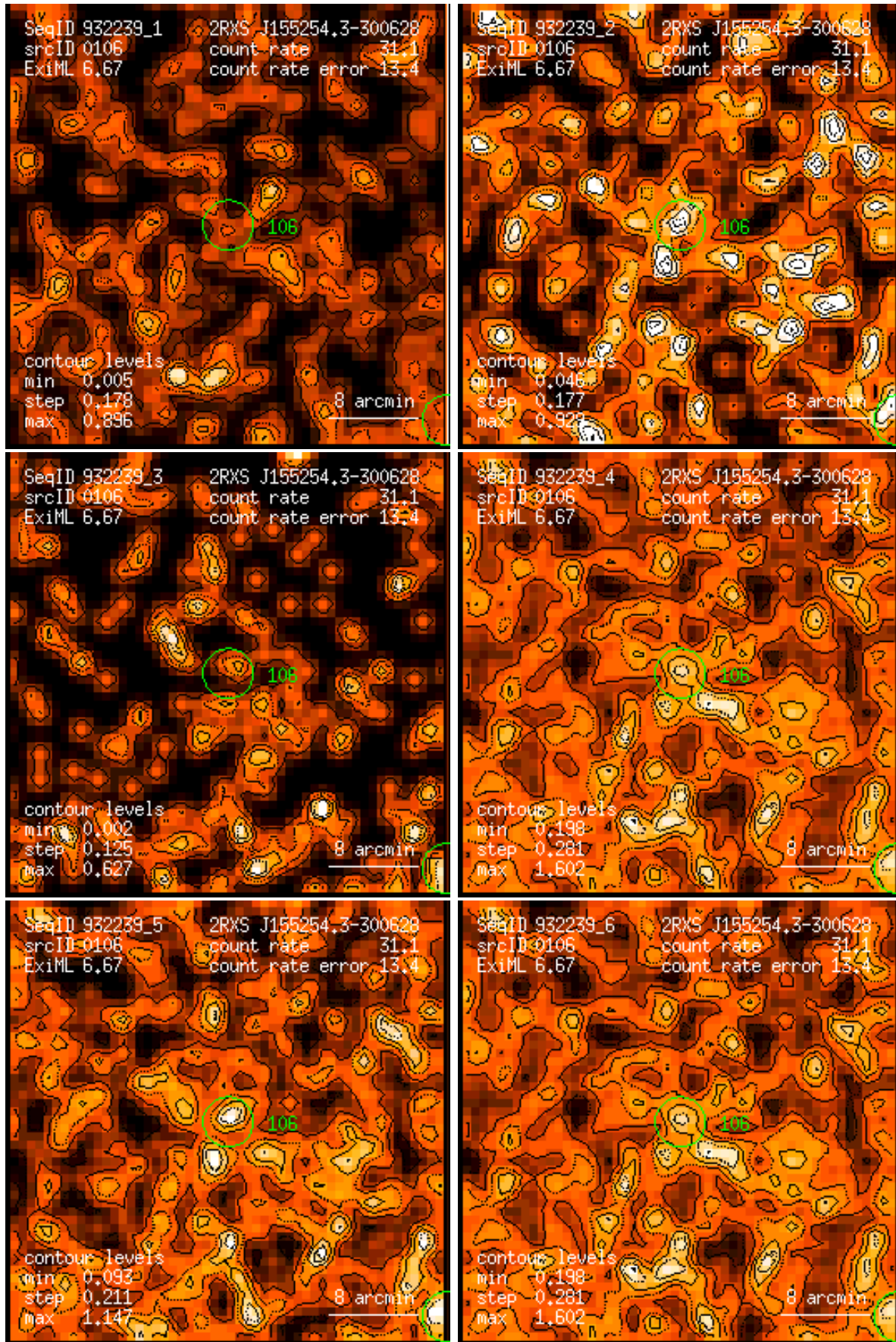
Figure 106: RASS 932239: detection 0106: band rate images, Gaussian filter: (1) PSPC channels 11 – 41, (2) 52 – 90, (3) 91 – 201, (4) 11 – 235, (5) 52 – 201, (6) 11 – 201. Broad band rates in counts/ks. Band rate contour levels in counts/ks/arcmin 2 .
