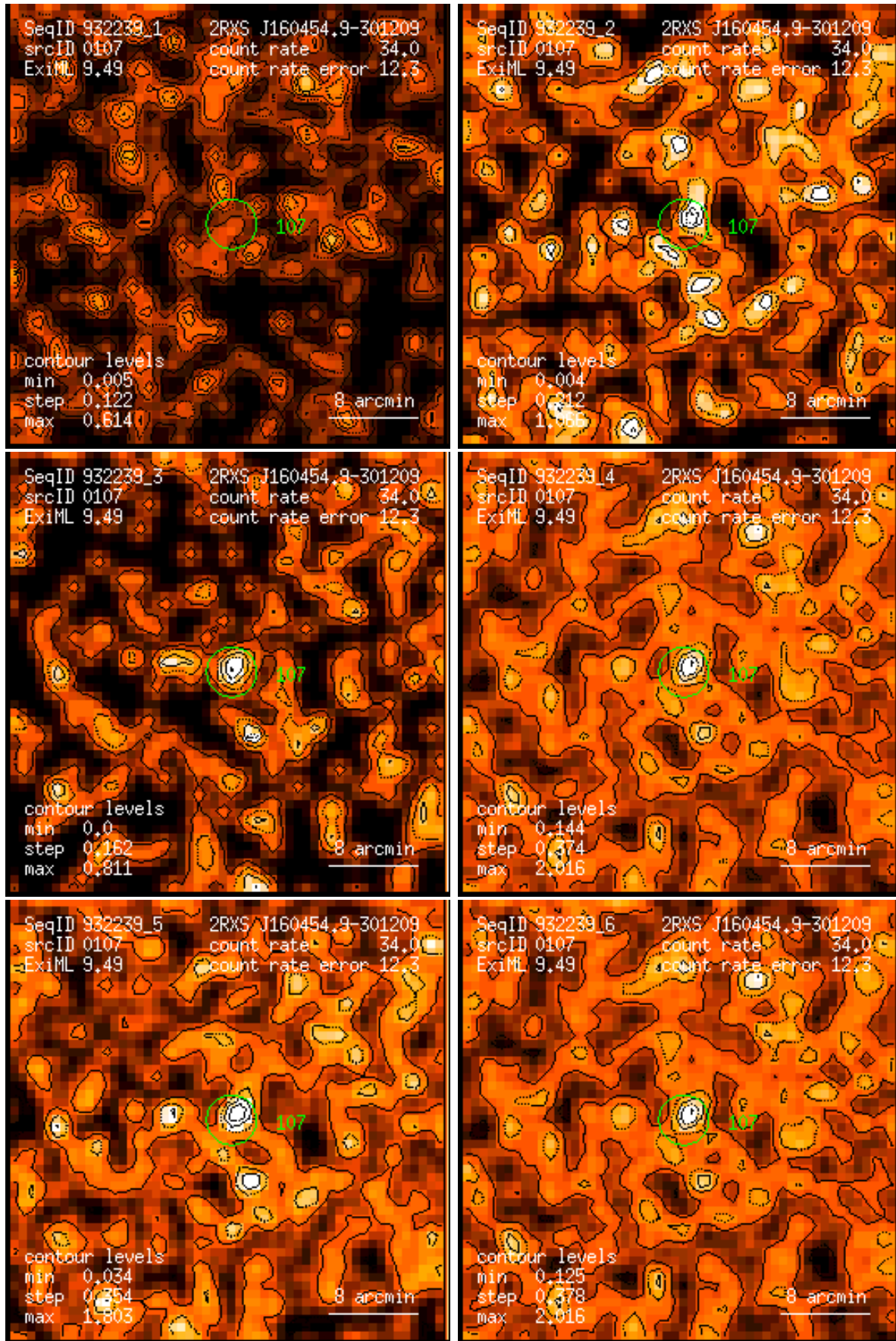
Figure 107: RASS 932239: detection 0107: band rate images, Gaussian filter: (1) PSPC channels 11 – 41, (2) 52 – 90, (3) 91 – 201, (4) 11 – 235, (5) 52 – 201, (6) 11 – 201. Broad band rates in counts/ks. Band rate contour levels in counts/ks/arcmin 2 .
