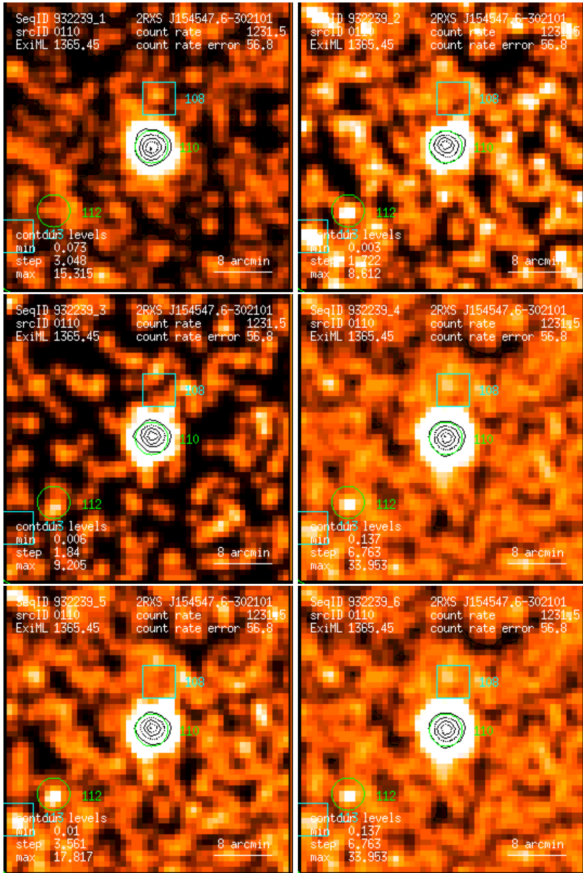
Figure 110: RASS 932239: detection 0110: band rate images, Gaussian filter: (1) PSPC channels 11 – 41, (2) 52 – 90, (3) 91 – 201, (4) 11 – 235, (5) 52 – 201, (6) 11 – 201. Broad band rates in counts/ks. Band rate contour levels in counts/ks/arcmin 2 .
