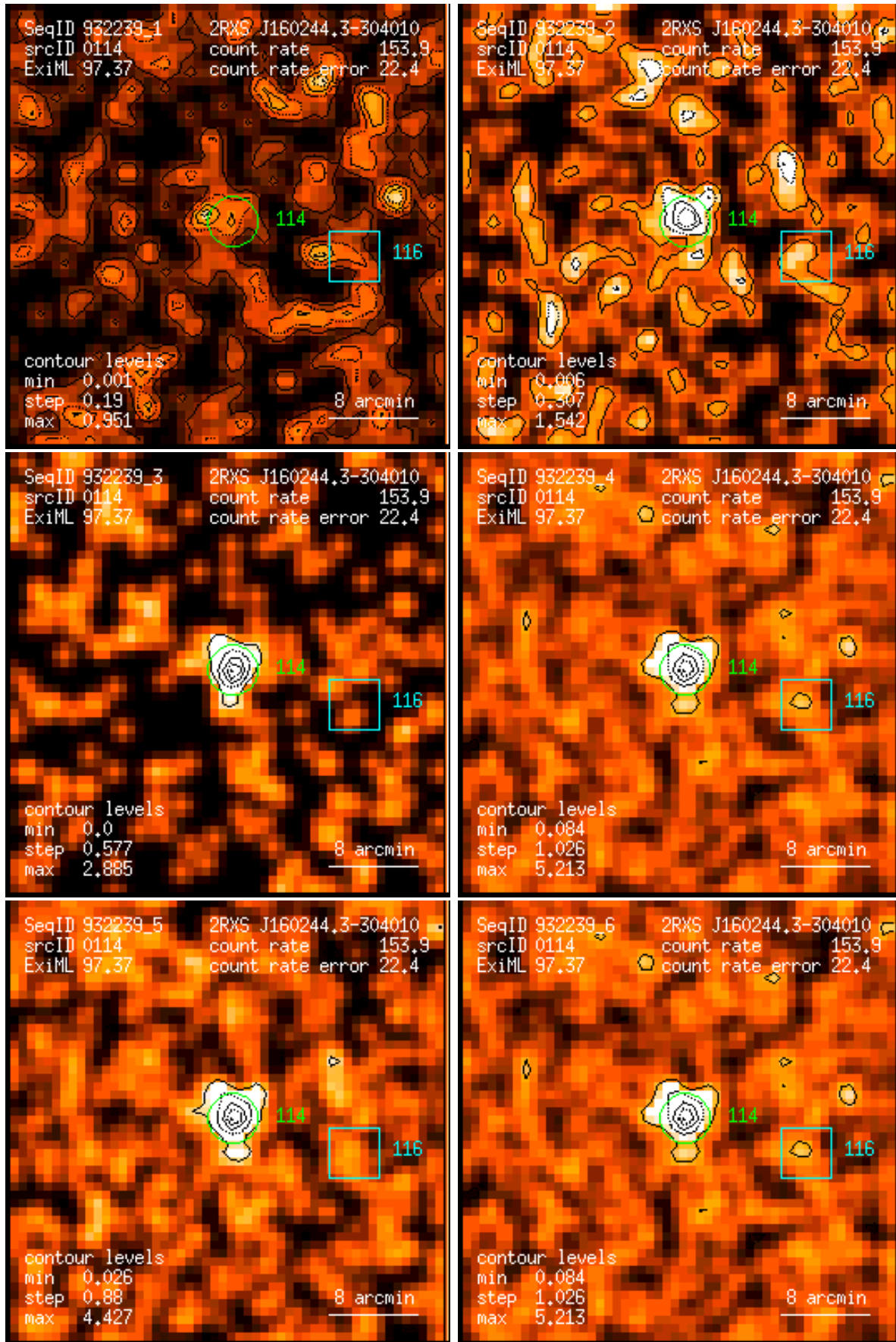
Figure 114: RASS 932239: detection 0114: band rate images, Gaussian filter: (1) PSPC channels 11 – 41, (2) 52 – 90, (3) 91 – 201, (4) 11 – 235, (5) 52 – 201, (6) 11 – 201. Broad band rates in counts/ks. Band rate contour levels in counts/ks/arcmin 2 .
