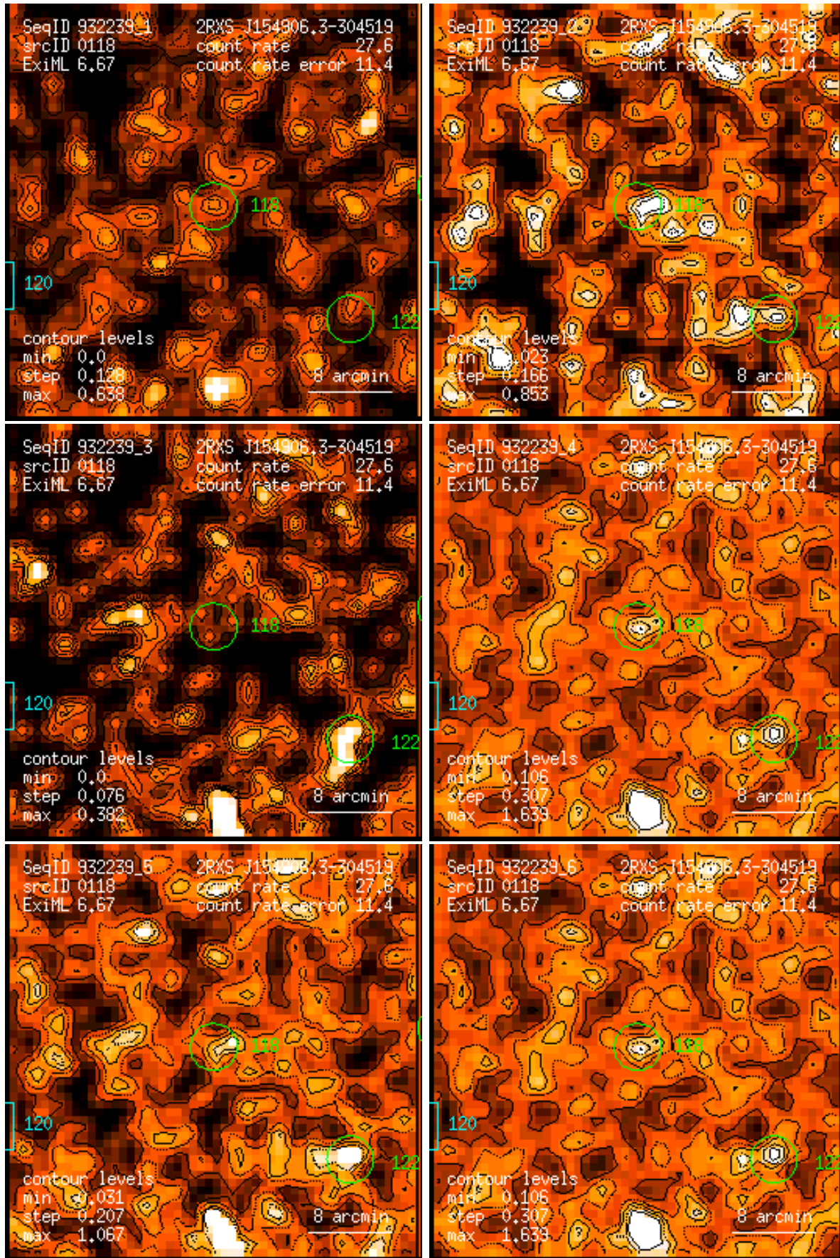
Figure 118: RASS 932239: detection 0118: band rate images, Gaussian filter: (1) PSPC channels 11 – 41, (2) 52 – 90, (3) 91 – 201, (4) 11 – 235, (5) 52 – 201, (6) 11 – 201. Broad band rates in counts/ks. Band rate contour levels in counts/ks/arcmin 2 .
