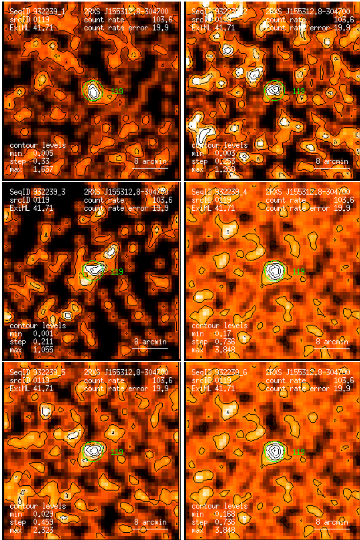
Figure 119: RASS 932239: detection 0119: band rate images, Gaussian filter: (1) PSPC channels 11 – 41, (2) 52 – 90, (3) 91 – 201, (4) 11 – 235, (5) 52 – 201, (6) 11 – 201. Broad band rates in counts/ks. Band rate contour levels in counts/ks/arcmin 2 .
