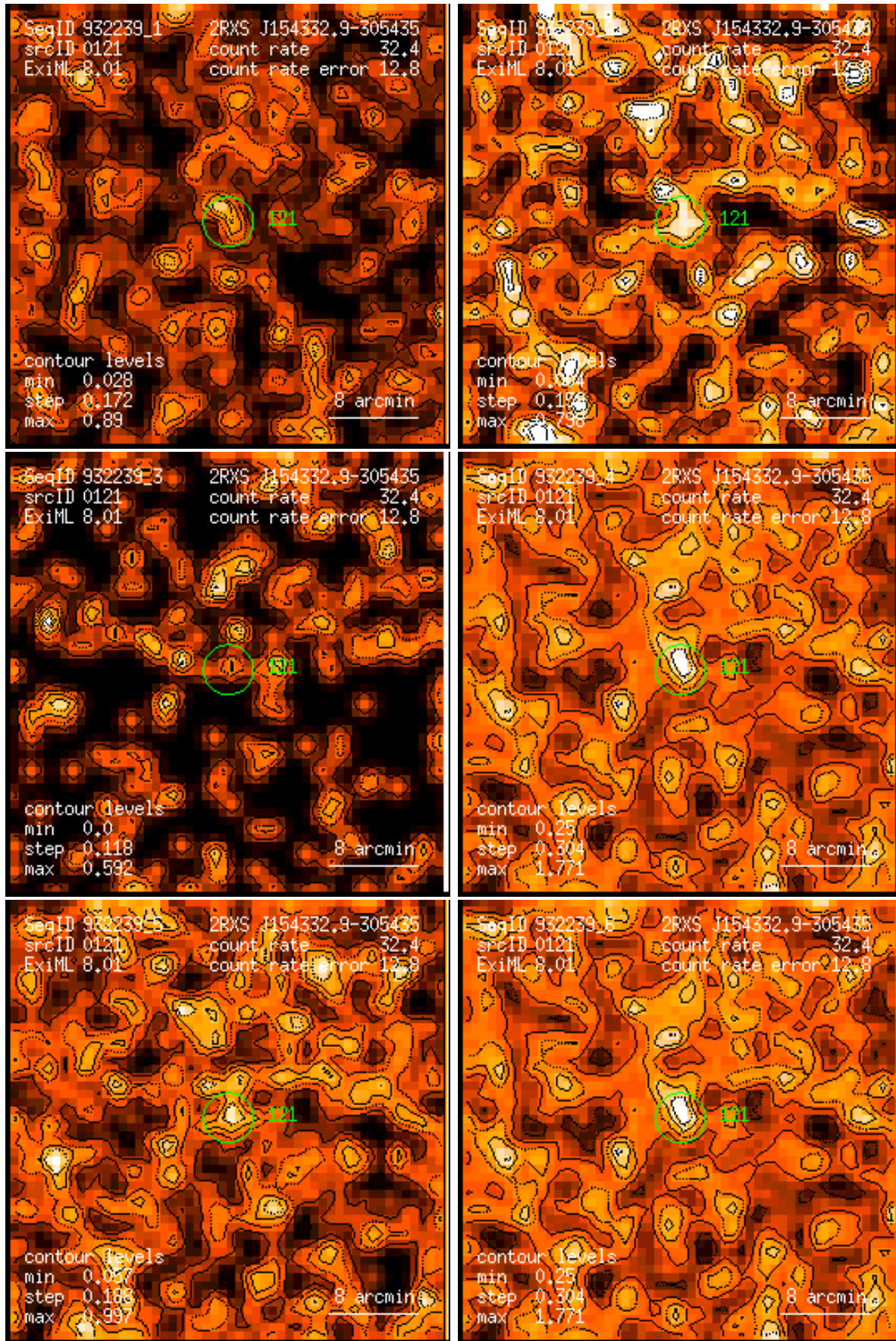
Figure 121: RASS 932239: detection 0121: band rate images, Gaussian filter: (1) PSPC channels 11 – 41, (2) 52 – 90, (3) 91 – 201, (4) 11 – 235, (5) 52 – 201, (6) 11 – 201. Broad band rates in counts/ks. Band rate contour levels in counts/ks/arcmin 2 .
