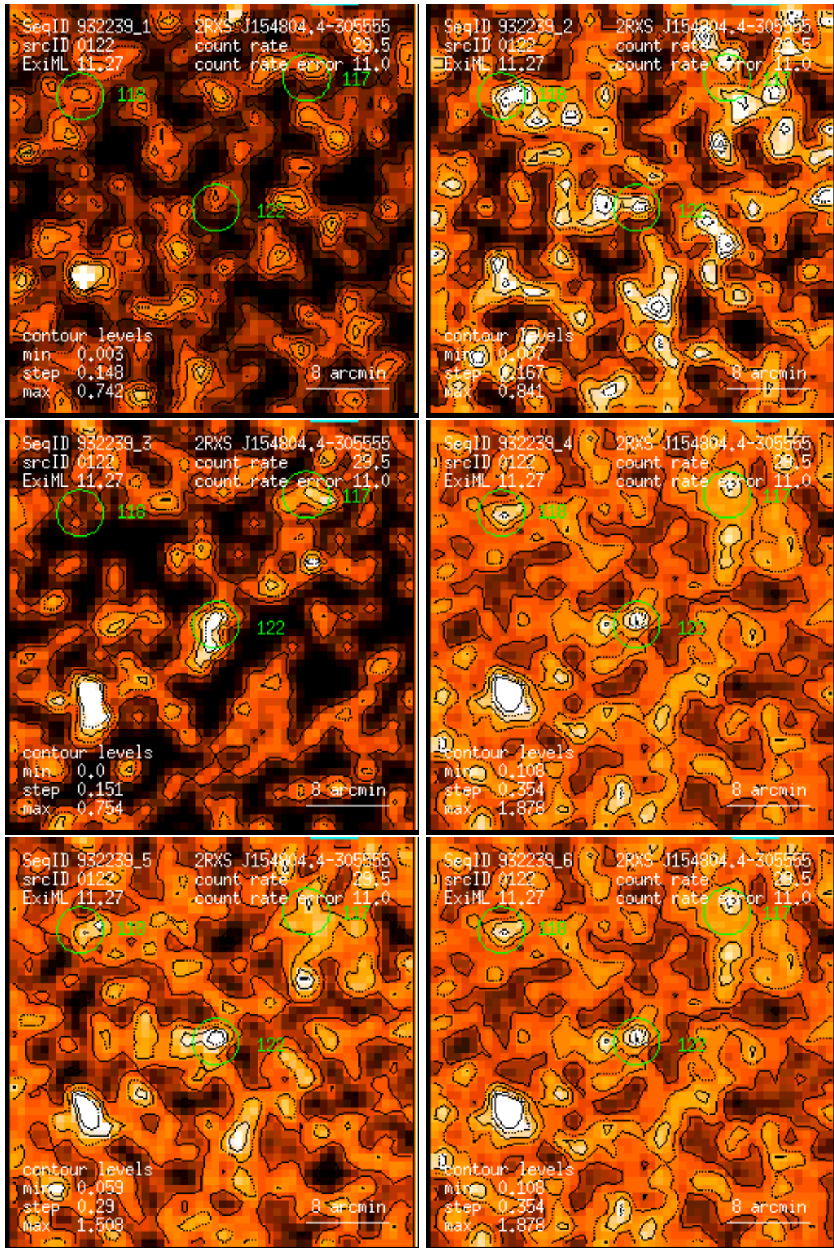
Figure 122: RASS 932239: detection 0122: band rate images, Gaussian filter: (1) PSPC channels 11 – 41, (2) 52 – 90, (3) 91 – 201, (4) 11 – 235, (5) 52 – 201, (6) 11 – 201. Broad band rates in counts/ks. Band rate contour levels in counts/ks/arcmin 2 .
