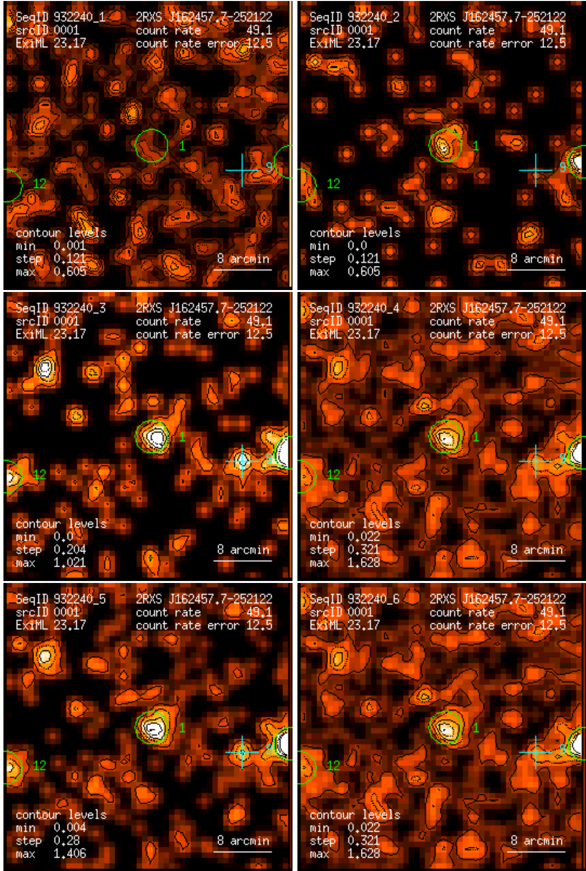
Figure 1: RASS 932240: detection 0001: band rate images, Gaussian filter: (1) PSPC channels 11 – 41, (2) 52 – 90, (3) 91 – 201, (4) 11 – 235, (5) 52 – 201, (6) 11 – 201. Broad band rates in counts/ks. Band rate contour levels in counts/ks/arcmin 2 .
