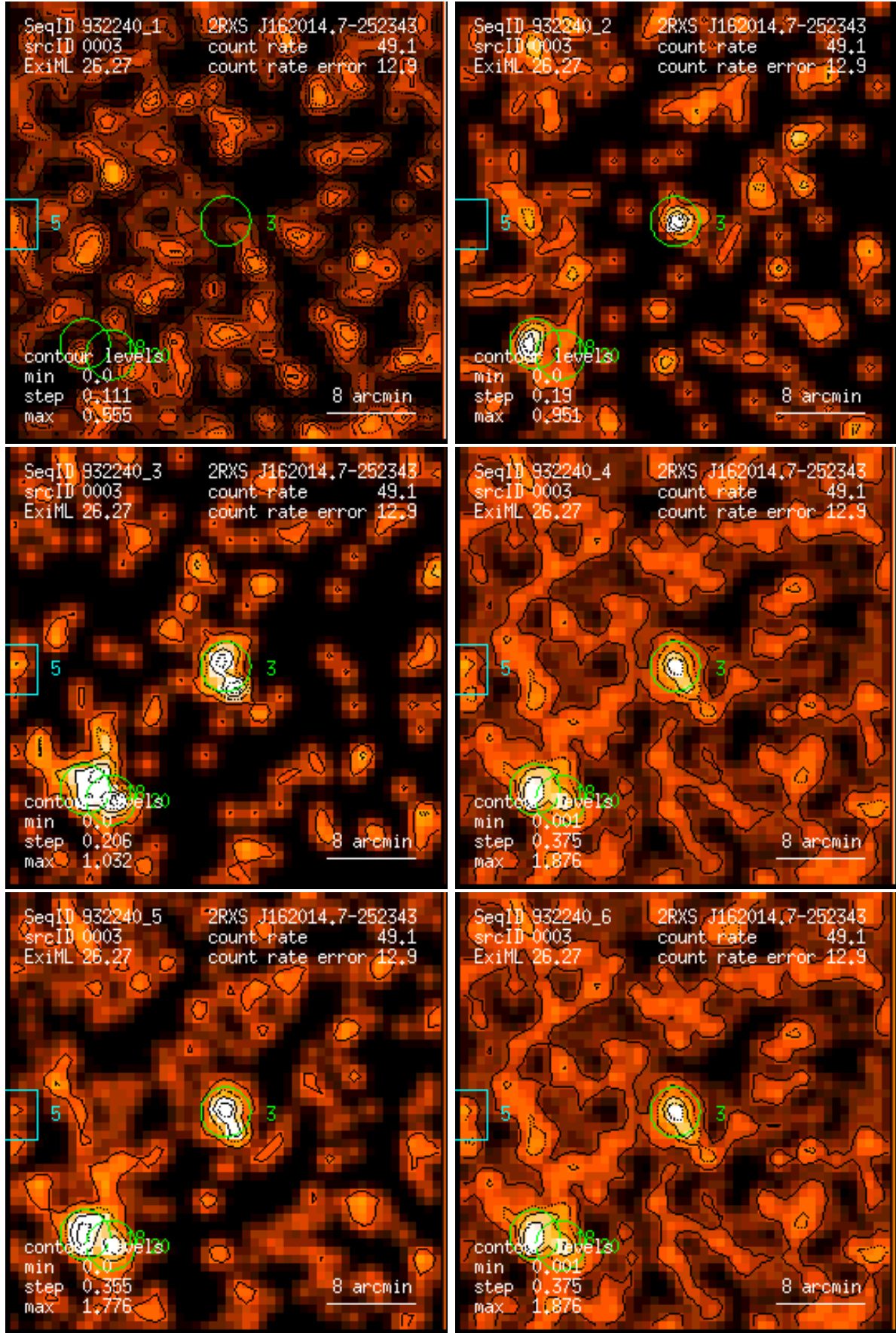
Figure 3: RASS 932240: detection 0003: band rate images, Gaussian filter: (1) PSPC channels 11 – 41, (2) 52 – 90, (3) 91 – 201, (4) 11 – 235, (5) 52 – 201, (6) 11 – 201. Broad band rates in counts/ks. Band rate contour levels in counts/ks/arcmin 2 .
