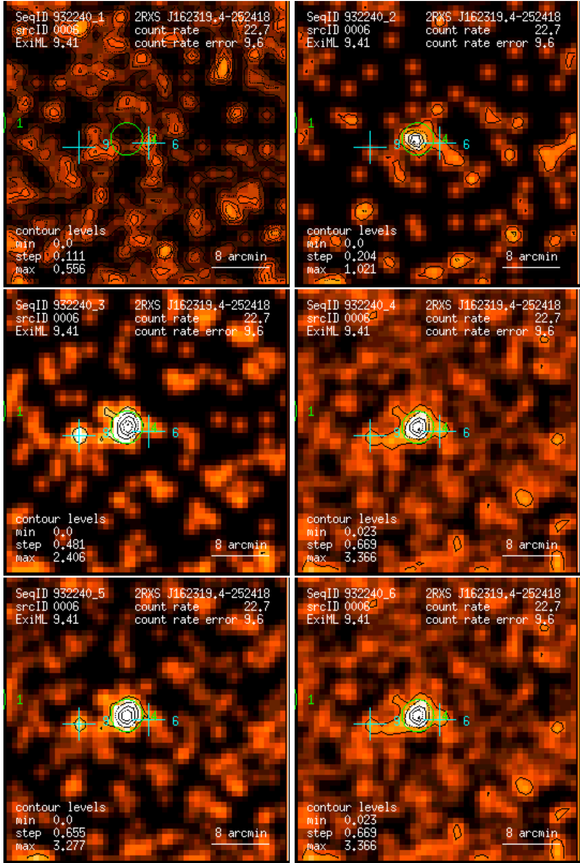
Figure 6: RASS 932240: detection 0006: band rate images, Gaussian filter: (1) PSPC channels 11 – 41, (2) 52 – 90, (3) 91 – 201, (4) 11 – 235, (5) 52 – 201, (6) 11 – 201. Broad band rates in counts/ks. Band rate contour levels in counts/ks/arcmin 2 .
