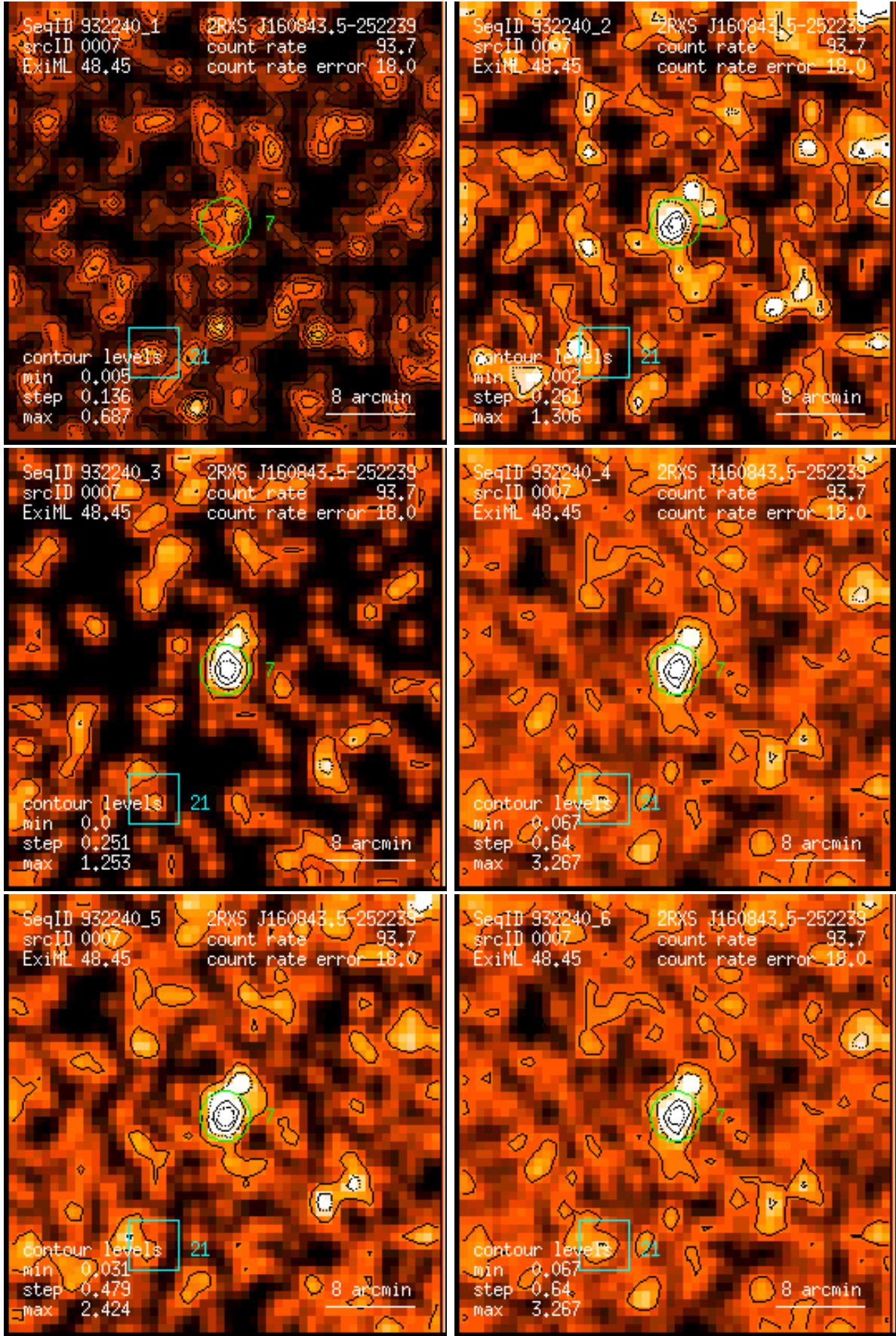
Figure 7: RASS 932240: detection 0007: band rate images, Gaussian filter: (1) PSPC channels 11 – 41, (2) 52 – 90, (3) 91 – 201, (4) 11 – 235, (5) 52 – 201, (6) 11 – 201. Broad band rates in counts/ks. Band rate contour levels in counts/ks/arcmin 2 .
