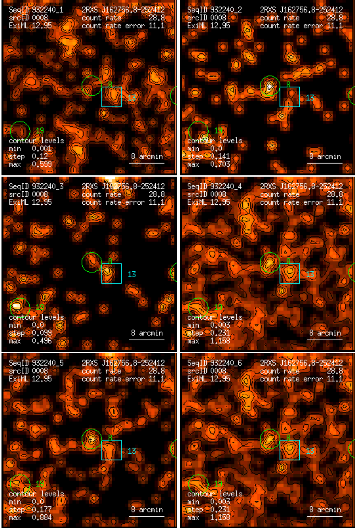
Figure 8: RASS 932240: detection 0008: band rate images, Gaussian filter: (1) PSPC channels 11 – 41, (2) 52 – 90, (3) 91 – 201, (4) 11 – 235, (5) 52 – 201, (6) 11 – 201. Broad band rates in counts/ks. Band rate contour levels in counts/ks/arcmin 2 .
