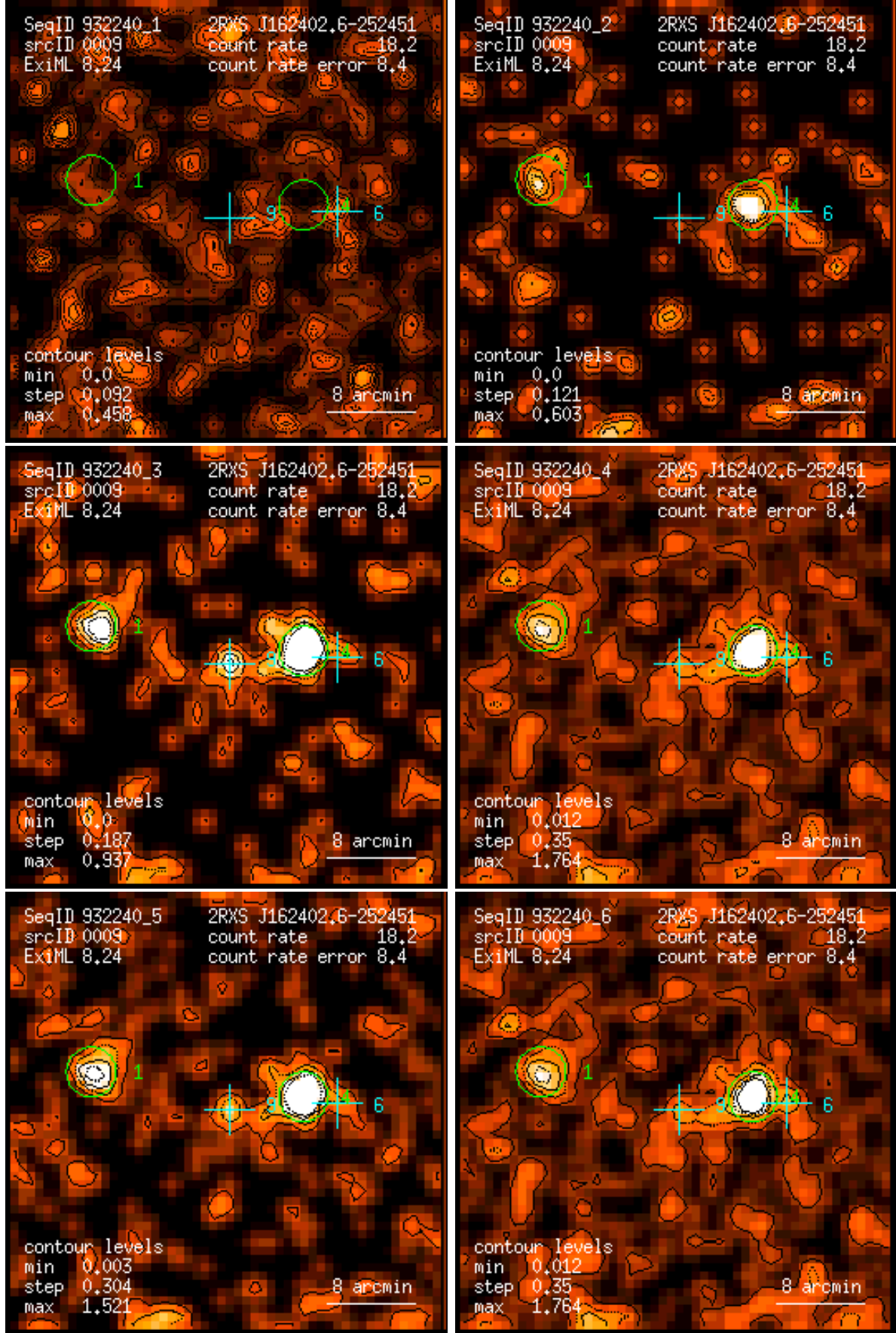
Figure 9: RASS 932240: detection 0009: band rate images, Gaussian filter: (1) PSPC channels 11 – 41, (2) 52 – 90, (3) 91 – 201, (4) 11 – 235, (5) 52 – 201, (6) 11 – 201. Broad band rates in counts/ks. Band rate contour levels in counts/ks/arcmin 2 .
