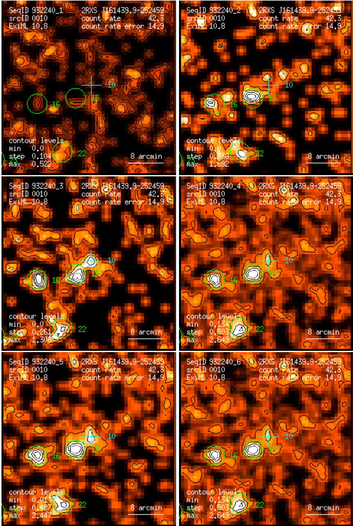
Figure 10: RASS 932240: detection 0010: band rate images, Gaussian filter: (1) PSPC channels 11 – 41, (2) 52 – 90, (3) 91 – 201, (4) 11 – 235, (5) 52 – 201, (6) 11 – 201. Broad band rates in counts/ks. Band rate contour levels in counts/ks/arcmin 2 .
