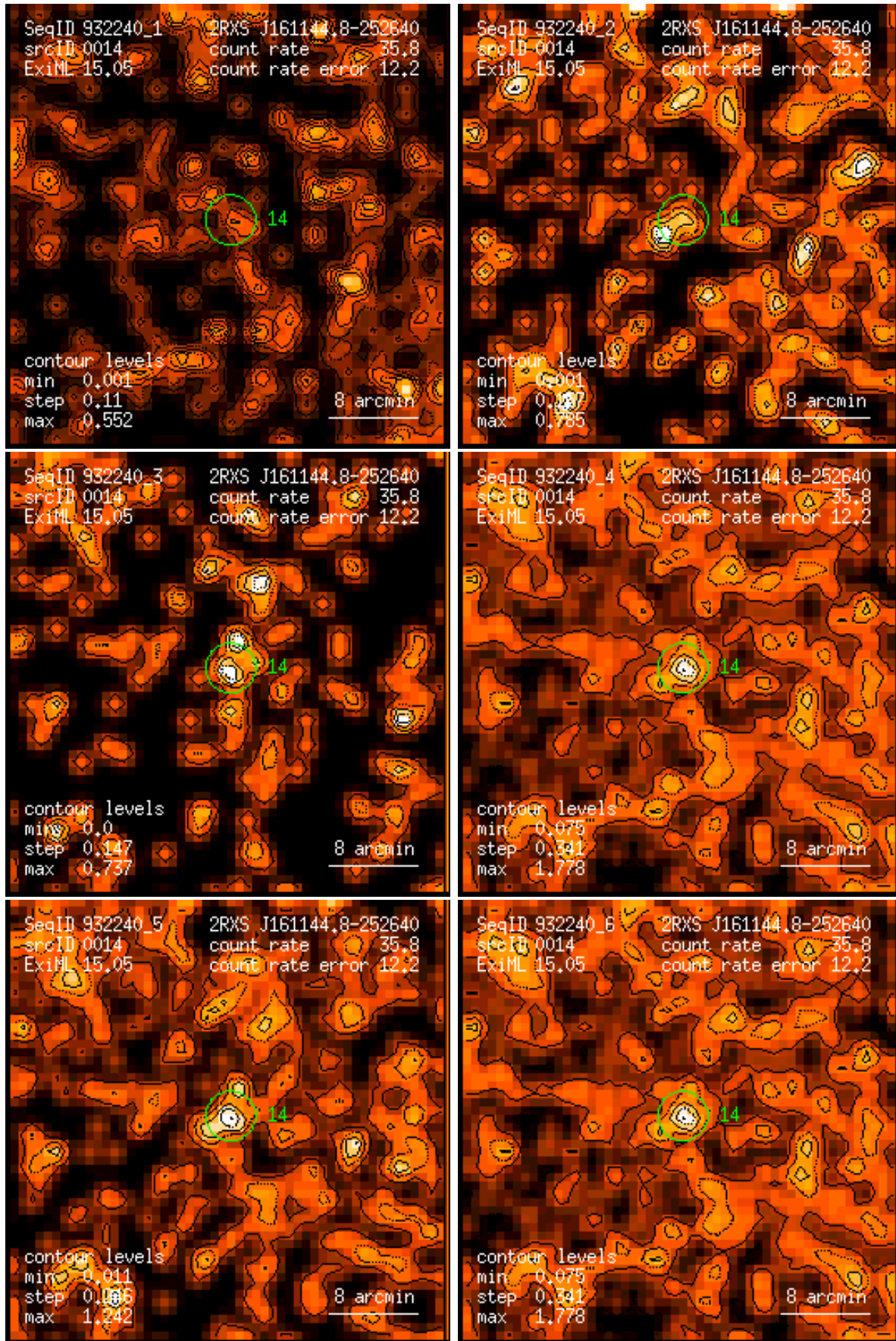
Figure 14: RASS 932240: detection 0014: band rate images, Gaussian filter: (1) PSPC channels 11 – 41, (2) 52 – 90, (3) 91 – 201, (4) 11 – 235, (5) 52 – 201, (6) 11 – 201. Broad band rates in counts/ks. Band rate contour levels in counts/ks/arcmin 2 .
