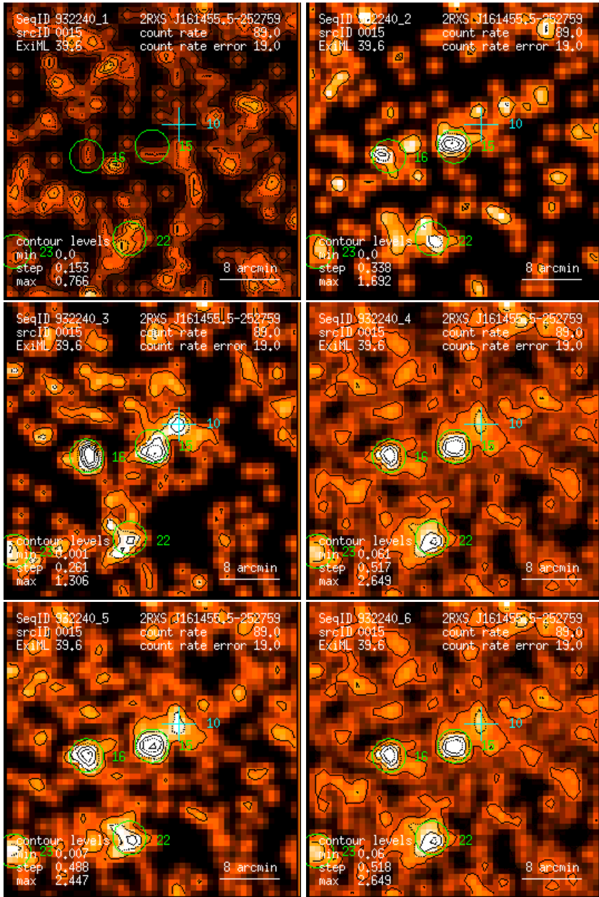
Figure 15: RASS 932240: detection 0015: band rate images, Gaussian filter: (1) PSPC channels 11 – 41, (2) 52 – 90, (3) 91 – 201, (4) 11 – 235, (5) 52 – 201, (6) 11 – 201. Broad band rates in counts/ks. Band rate contour levels in counts/ks/arcmin 2 .
