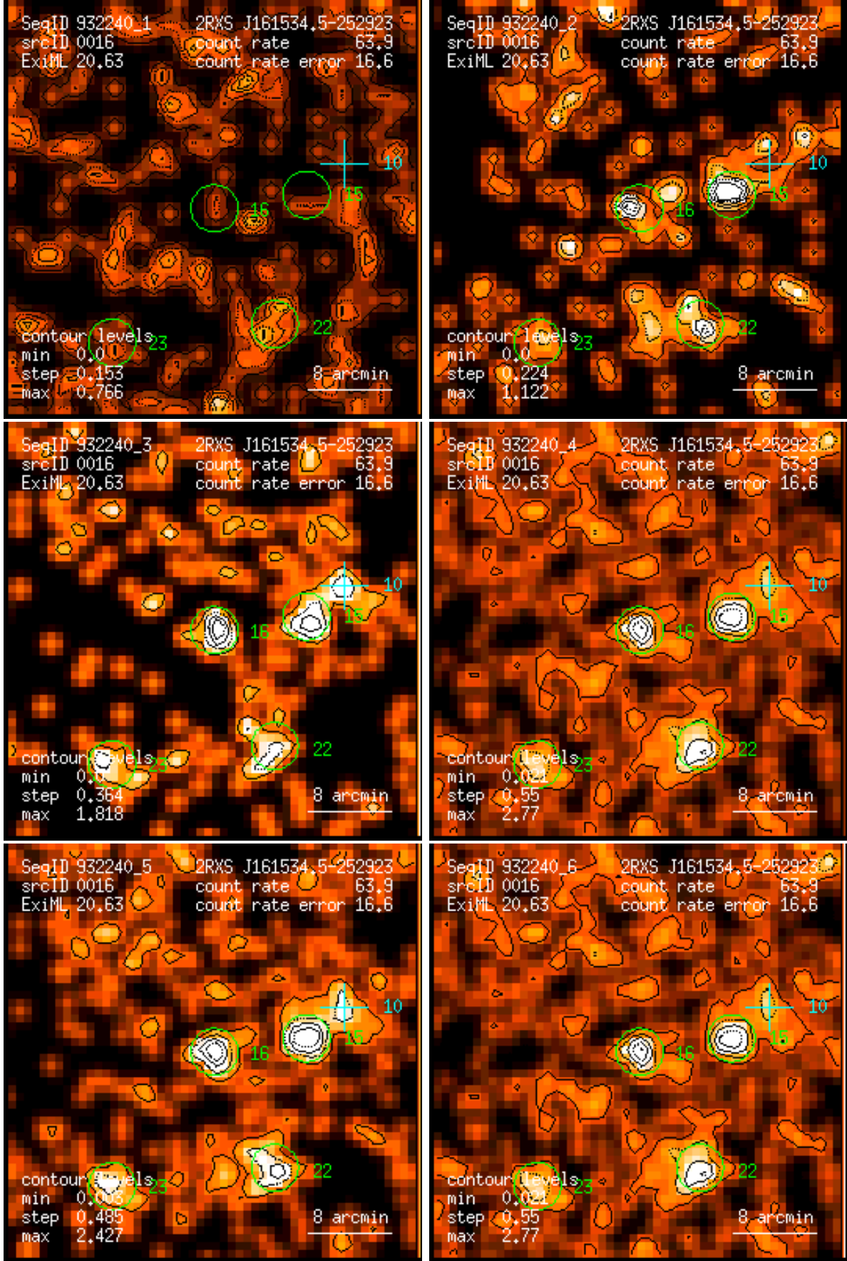
Figure 16: RASS 932240: detection 0016: band rate images, Gaussian filter: (1) PSPC channels 11 – 41, (2) 52 – 90, (3) 91 – 201, (4) 11 – 235, (5) 52 – 201, (6) 11 – 201. Broad band rates in counts/ks. Band rate contour levels in counts/ks/arcmin 2 .
