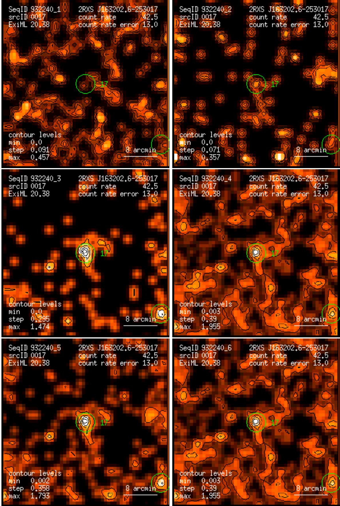
Figure 17: RASS 932240: detection 0017: band rate images, Gaussian filter: (1) PSPC channels 11 – 41, (2) 52 – 90, (3) 91 – 201, (4) 11 – 235, (5) 52 – 201, (6) 11 – 201. Broad band rates in counts/ks. Band rate contour levels in counts/ks/arcmin 2 .
