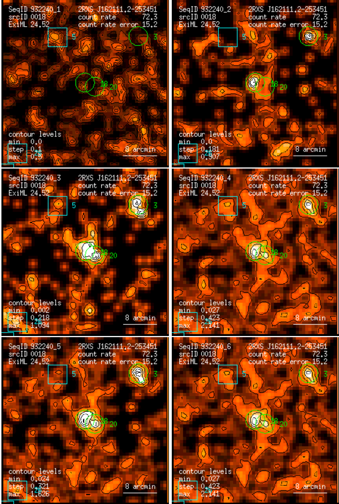
Figure 18: RASS 932240: detection 0018: band rate images, Gaussian filter: (1) PSPC channels 11 – 41, (2) 52 – 90, (3) 91 – 201, (4) 11 – 235, (5) 52 – 201, (6) 11 – 201. Broad band rates in counts/ks. Band rate contour levels in counts/ks/arcmin 2 .
