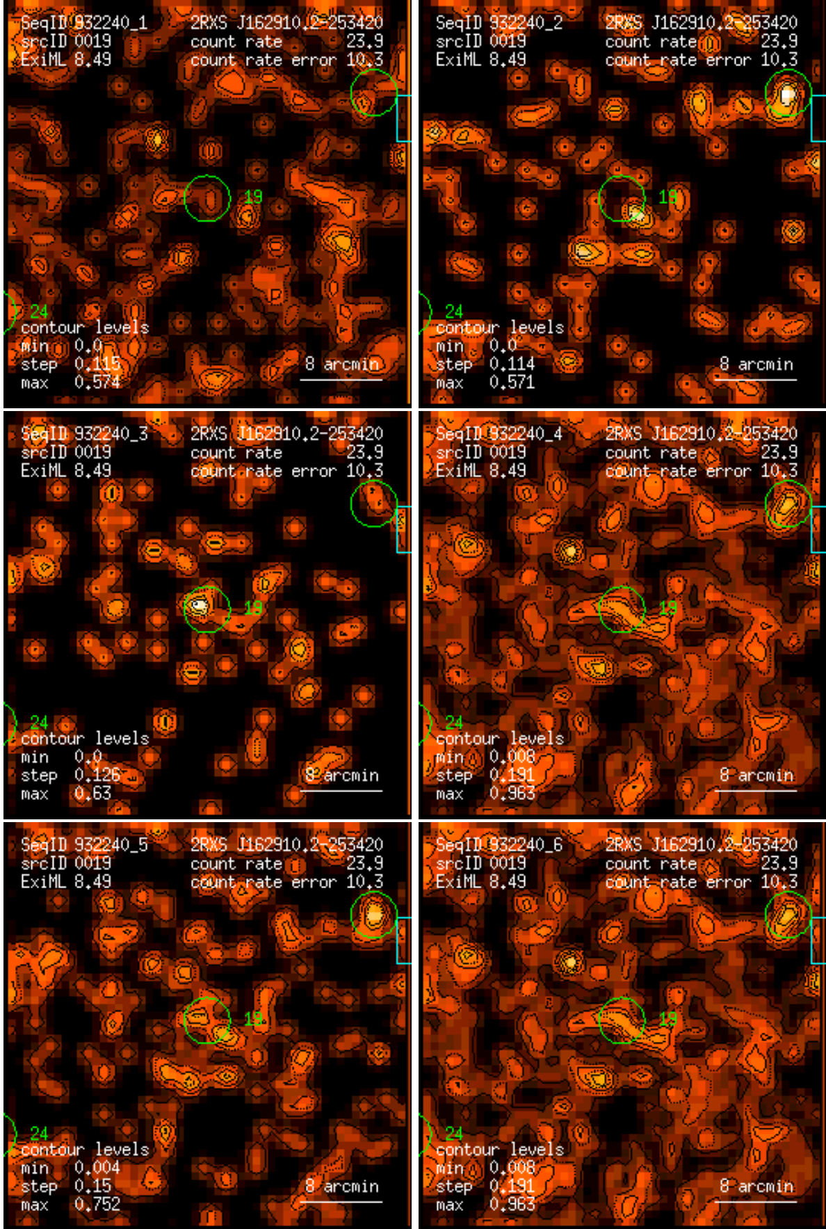
Figure 19: RASS 932240: detection 0019: band rate images, Gaussian filter: (1) PSPC channels 11 – 41, (2) 52 – 90, (3) 91 – 201, (4) 11 – 235, (5) 52 – 201, (6) 11 – 201. Broad band rates in counts/ks. Band rate contour levels in counts/ks/arcmin 2 .
