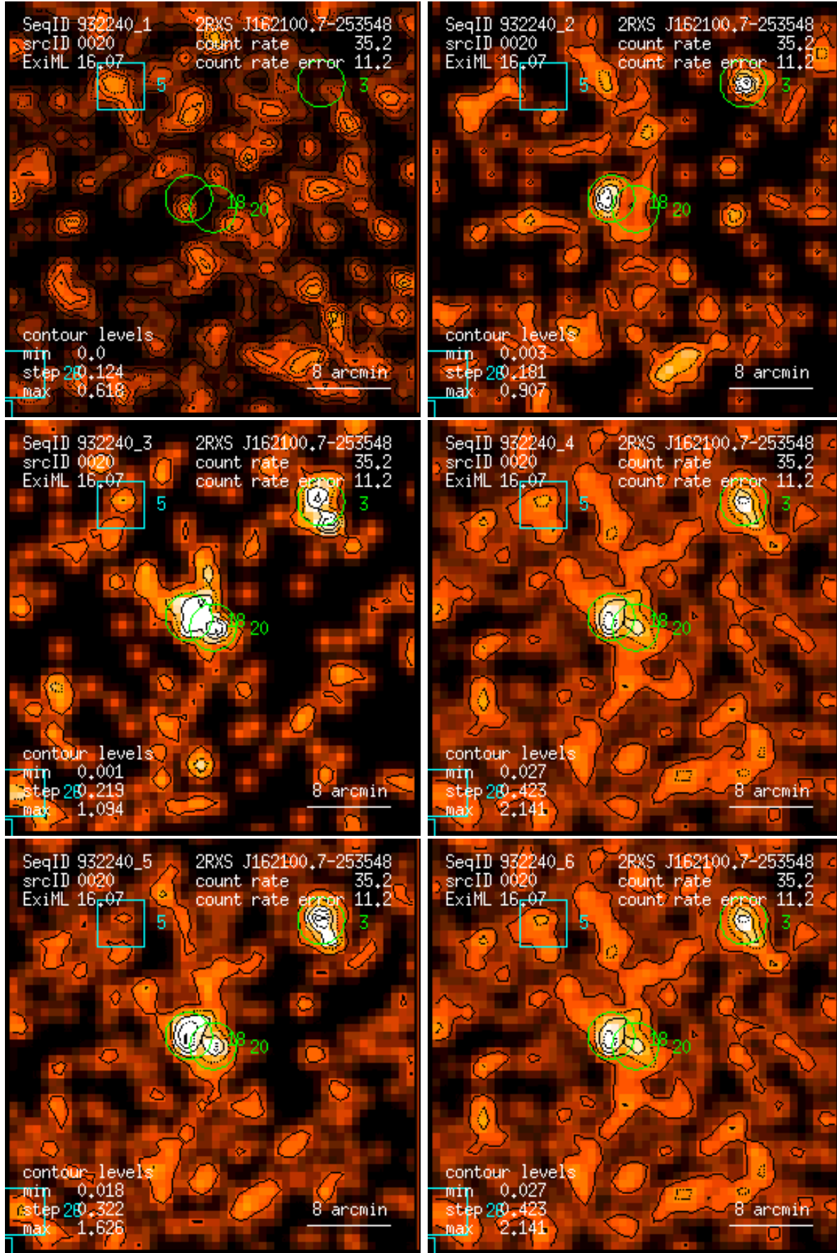
Figure 20: RASS 932240: detection 0020: band rate images, Gaussian filter: (1) PSPC channels 11 – 41, (2) 52 – 90, (3) 91 – 201, (4) 11 – 235, (5) 52 – 201, (6) 11 – 201. Broad band rates in counts/ks. Band rate contour levels in counts/ks/arcmin 2 .
