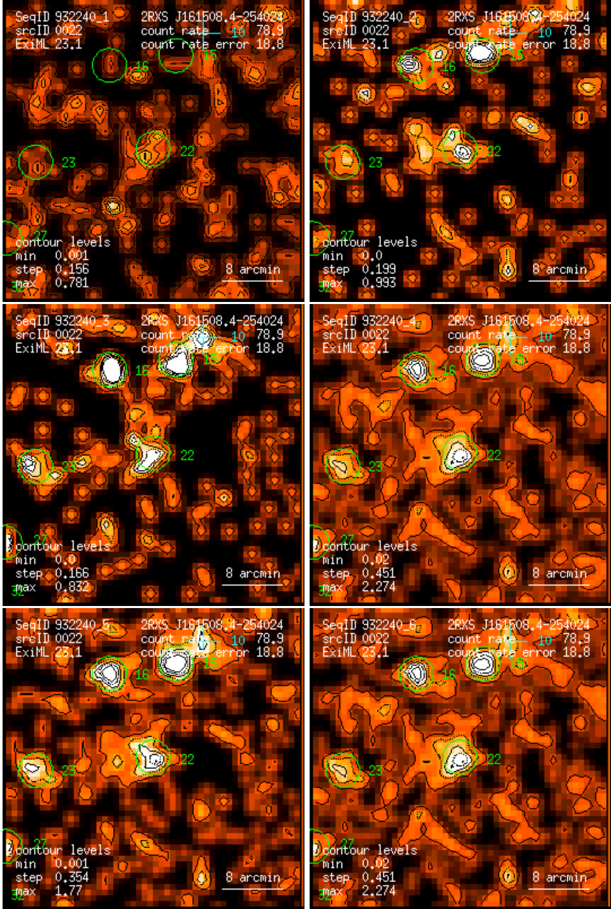
Figure 22: RASS 932240: detection 0022: band rate images, Gaussian filter: (1) PSPC channels 11 – 41, (2) 52 – 90, (3) 91 – 201, (4) 11 – 235, (5) 52 – 201, (6) 11 – 201. Broad band rates in counts/ks. Band rate contour levels in counts/ks/arcmin 2 .
