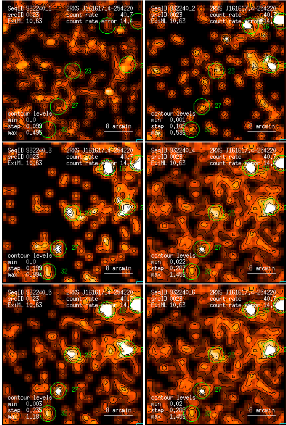
Figure 23: RASS 932240: detection 0023: band rate images, Gaussian filter: (1) PSPC channels 11 – 41, (2) 52 – 90, (3) 91 – 201, (4) 11 – 235, (5) 52 – 201, (6) 11 – 201. Broad band rates in counts/ks. Band rate contour levels in counts/ks/arcmin 2 .
