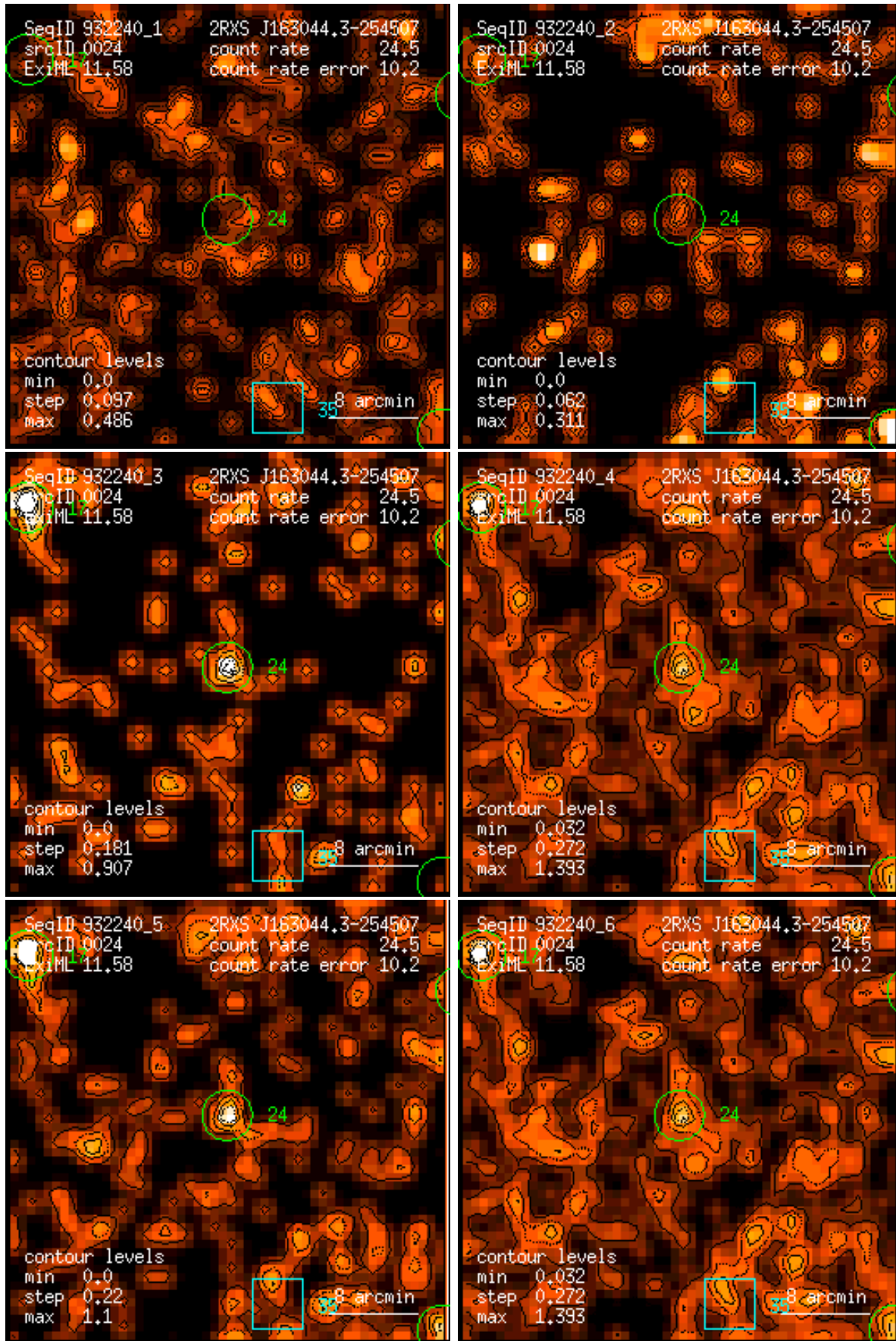
Figure 24: RASS 932240: detection 0024: band rate images, Gaussian filter: (1) PSPC channels 11 – 41, (2) 52 – 90, (3) 91 – 201, (4) 11 – 235, (5) 52 – 201, (6) 11 – 201. Broad band rates in counts/ks. Band rate contour levels in counts/ks/arcmin 2 .
