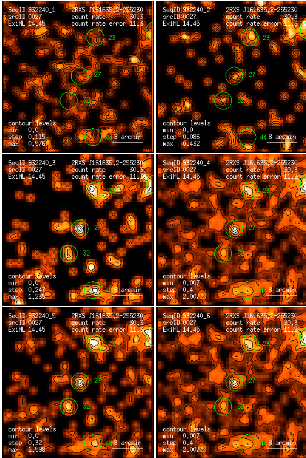
Figure 27: RASS 932240: detection 0027: band rate images, Gaussian filter: (1) PSPC channels 11 – 41, (2) 52 – 90, (3) 91 – 201, (4) 11 – 235, (5) 52 – 201, (6) 11 – 201. Broad band rates in counts/ks. Band rate contour levels in counts/ks/arcmin 2 .
