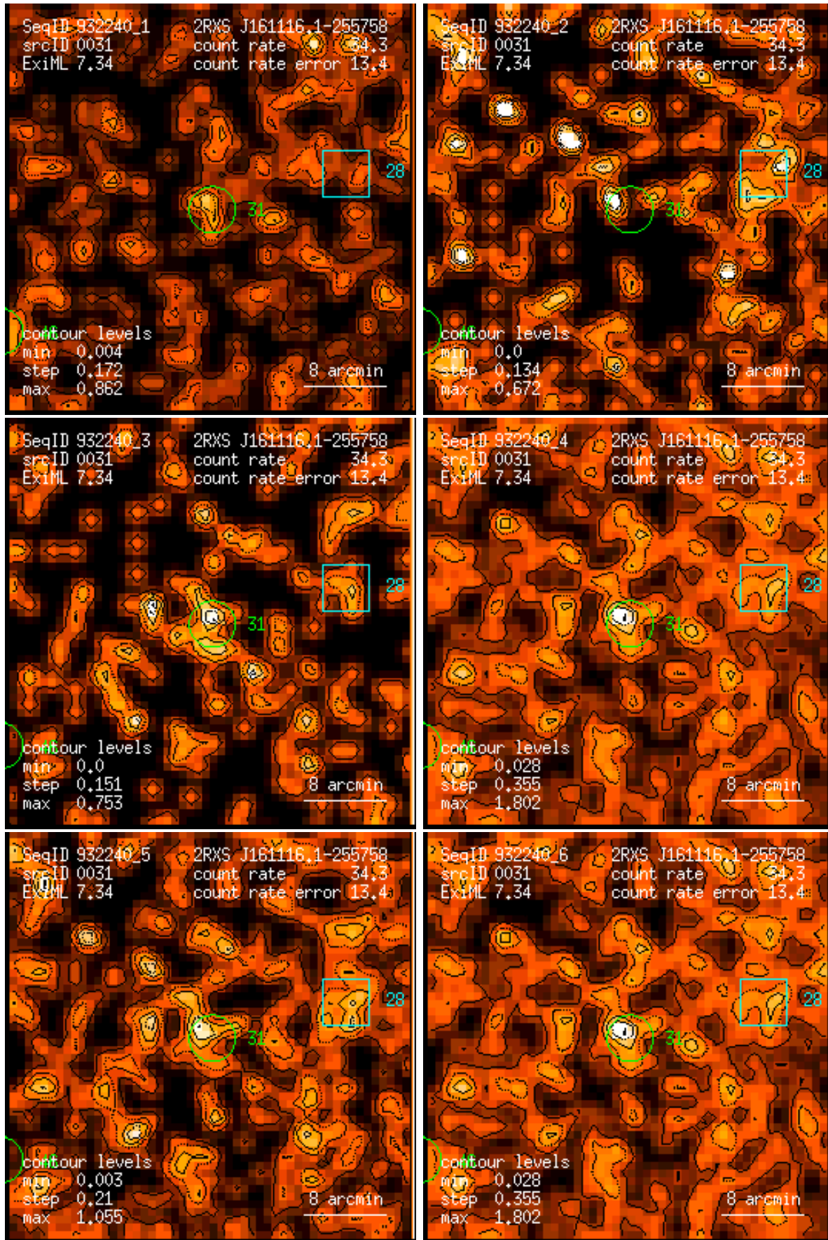
Figure 31: RASS 932240: detection 0031: band rate images, Gaussian filter: (1) PSPC channels 11 – 41, (2) 52 – 90, (3) 91 – 201, (4) 11 – 235, (5) 52 – 201, (6) 11 – 201. Broad band rates in counts/ks. Band rate contour levels in counts/ks/arcmin 2 .
