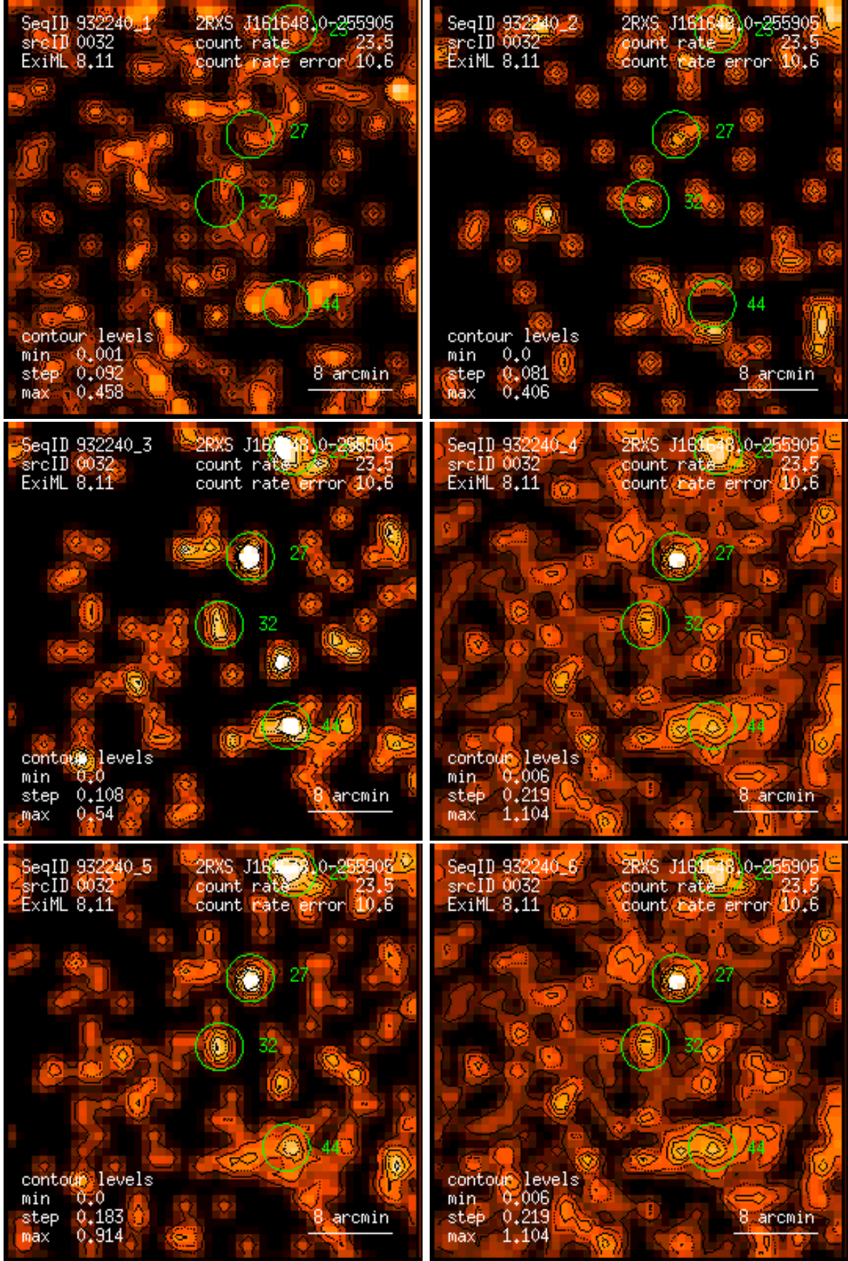
Figure 32: RASS 932240: detection 0032: band rate images, Gaussian filter: (1) PSPC channels 11 – 41, (2) 52 – 90, (3) 91 – 201, (4) 11 – 235, (5) 52 – 201, (6) 11 – 201. Broad band rates in counts/ks. Band rate contour levels in counts/ks/arcmin 2 .
