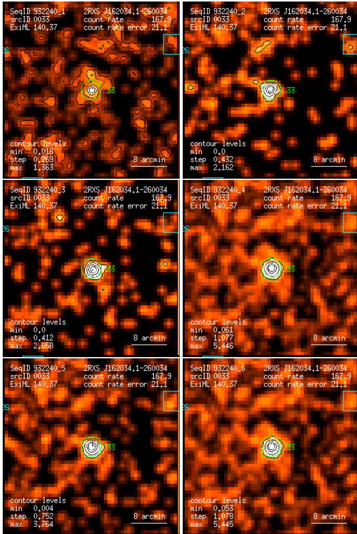
Figure 33: RASS 932240: detection 0033: band rate images, Gaussian filter: (1) PSPC channels 11 – 41, (2) 52 – 90, (3) 91 – 201, (4) 11 – 235, (5) 52 – 201, (6) 11 – 201. Broad band rates in counts/ks. Band rate contour levels in counts/ks/arcmin 2 .
