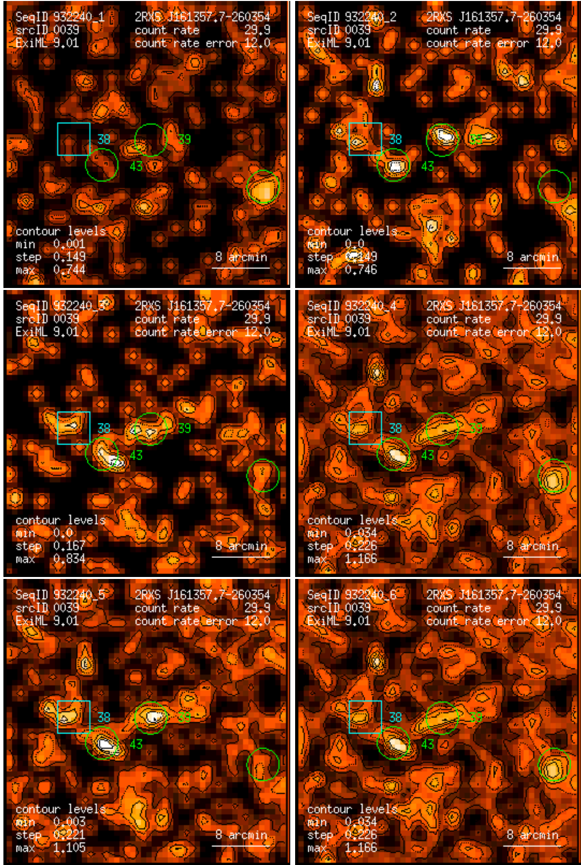
Figure 39: RASS 932240: detection 0039: band rate images, Gaussian filter: (1) PSPC channels 11 – 41, (2) 52 – 90, (3) 91 – 201, (4) 11 – 235, (5) 52 – 201, (6) 11 – 201. Broad band rates in counts/ks. Band rate contour levels in counts/ks/arcmin 2 .
